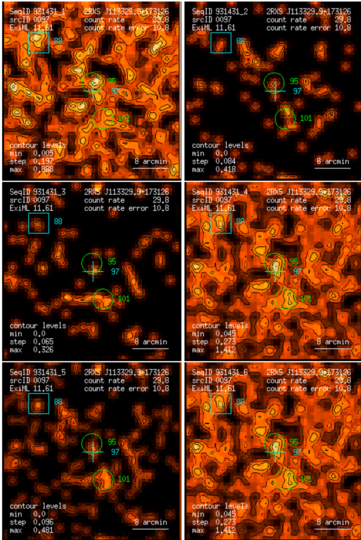
Figure 97: RASS 931431: detection 0097: band rate images, Gaussian filter: (1) PSPC channels 11 – 41, (2) 52 – 90, (3) 91 – 201, (4) 11 – 235, (5) 52 – 201, (6) 11 – 201. Broad band rates in counts/ks. Band rate contour levels in counts/ks/arcmin 2 .
