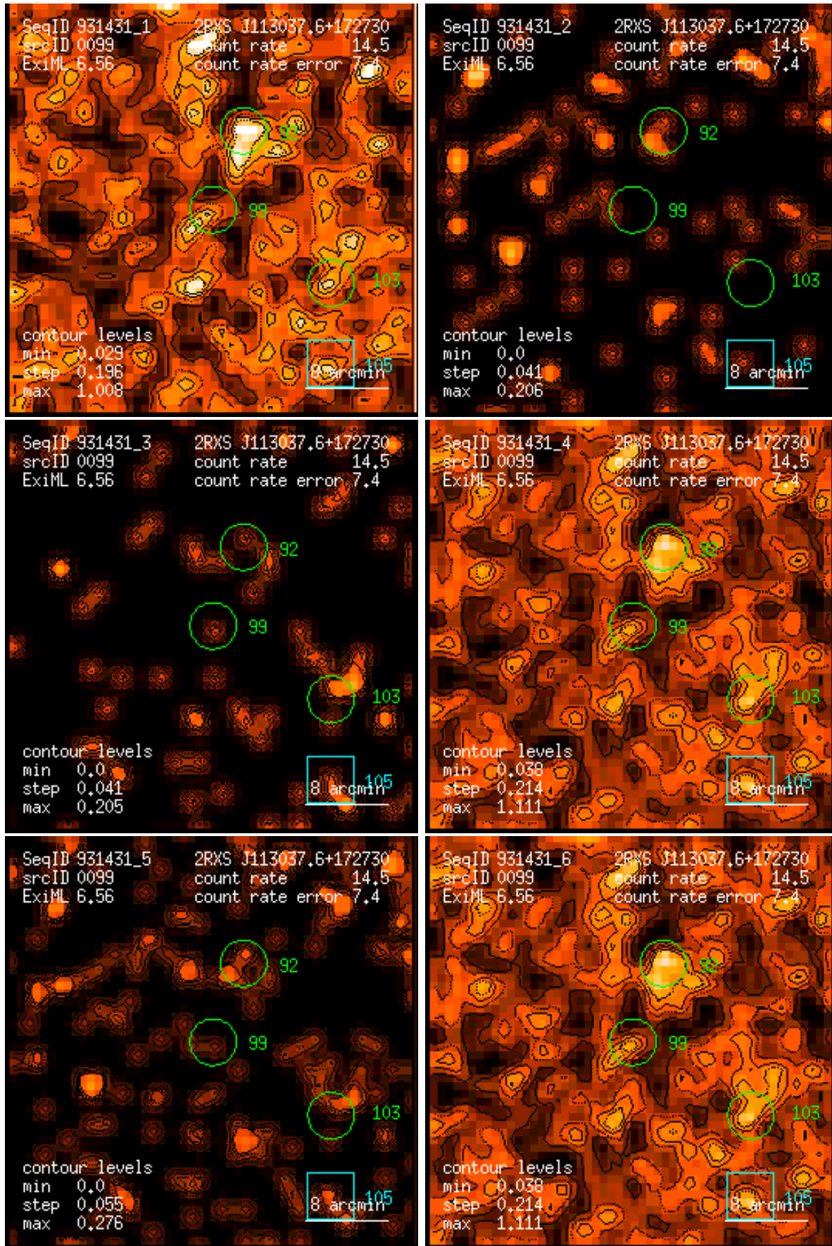
Figure 99: RASS 931431: detection 0099: band rate images, Gaussian filter: (1) PSPC channels 11 – 41, (2) 52 – 90, (3) 91 – 201, (4) 11 – 235, (5) 52 – 201, (6) 11 – 201. Broad band rates in counts/ks. Band rate contour levels in counts/ks/arcmin 2 .
