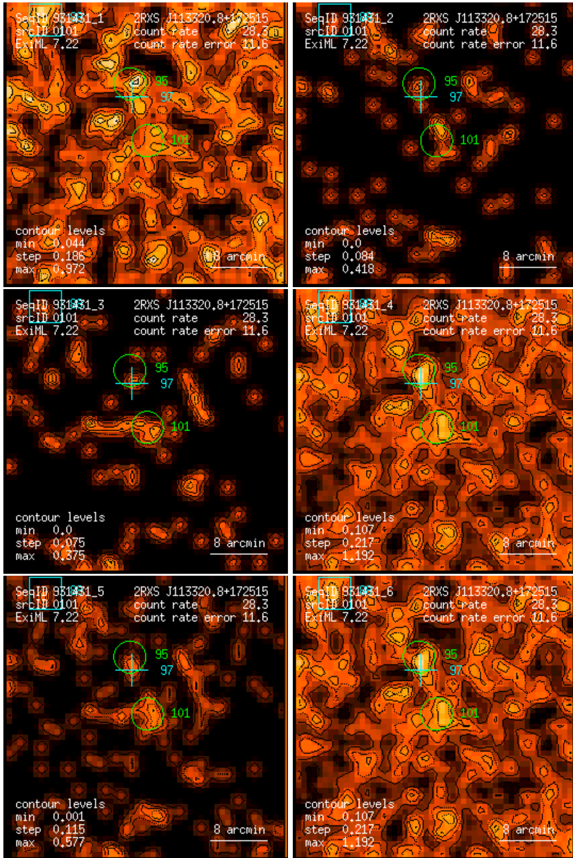
Figure 101: RASS 931431: detection 0101: band rate images, Gaussian filter: (1) PSPC channels 11 – 41, (2) 52 – 90, (3) 91 – 201, (4) 11 – 235, (5) 52 – 201, (6) 11 – 201. Broad band rates in counts/ks. Band rate contour levels in counts/ks/arcmin 2 .
