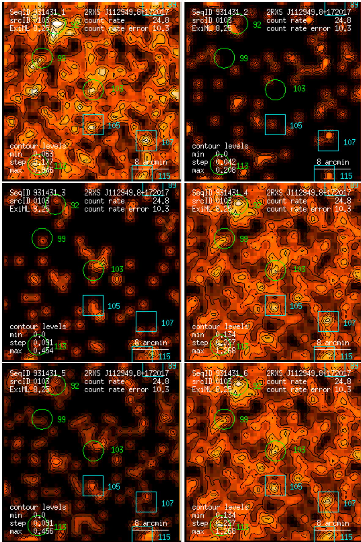
Figure 103: RASS 931431: detection 0103: band rate images, Gaussian filter: (1) PSPC channels 11 – 41, (2) 52 – 90, (3) 91 – 201, (4) 11 – 235, (5) 52 – 201, (6) 11 – 201. Broad band rates in counts/ks. Band rate contour levels in counts/ks/arcmin 2 .
