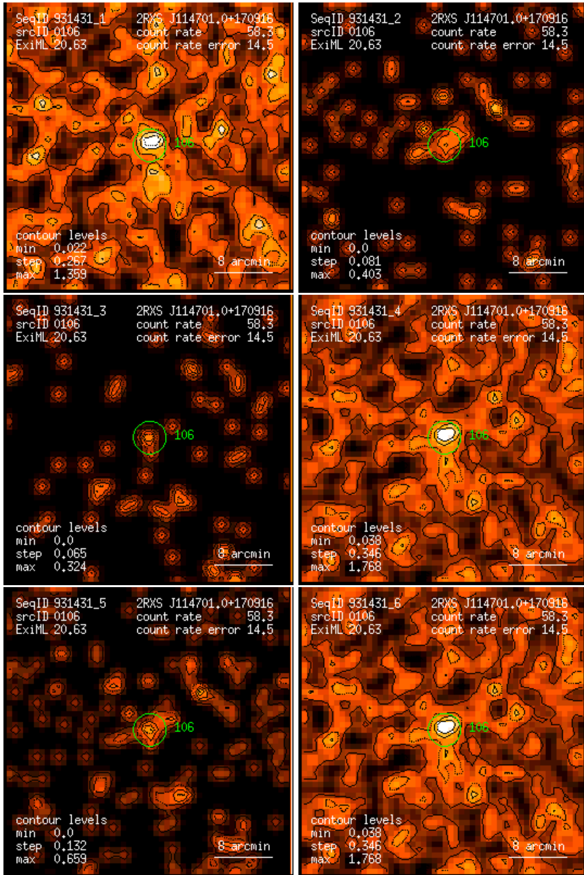
Figure 106: RASS 931431: detection 0106: band rate images, Gaussian filter: (1) PSPC channels 11 – 41, (2) 52 – 90, (3) 91 – 201, (4) 11 – 235, (5) 52 – 201, (6) 11 – 201. Broad band rates in counts/ks. Band rate contour levels in counts/ks/arcmin 2 .
