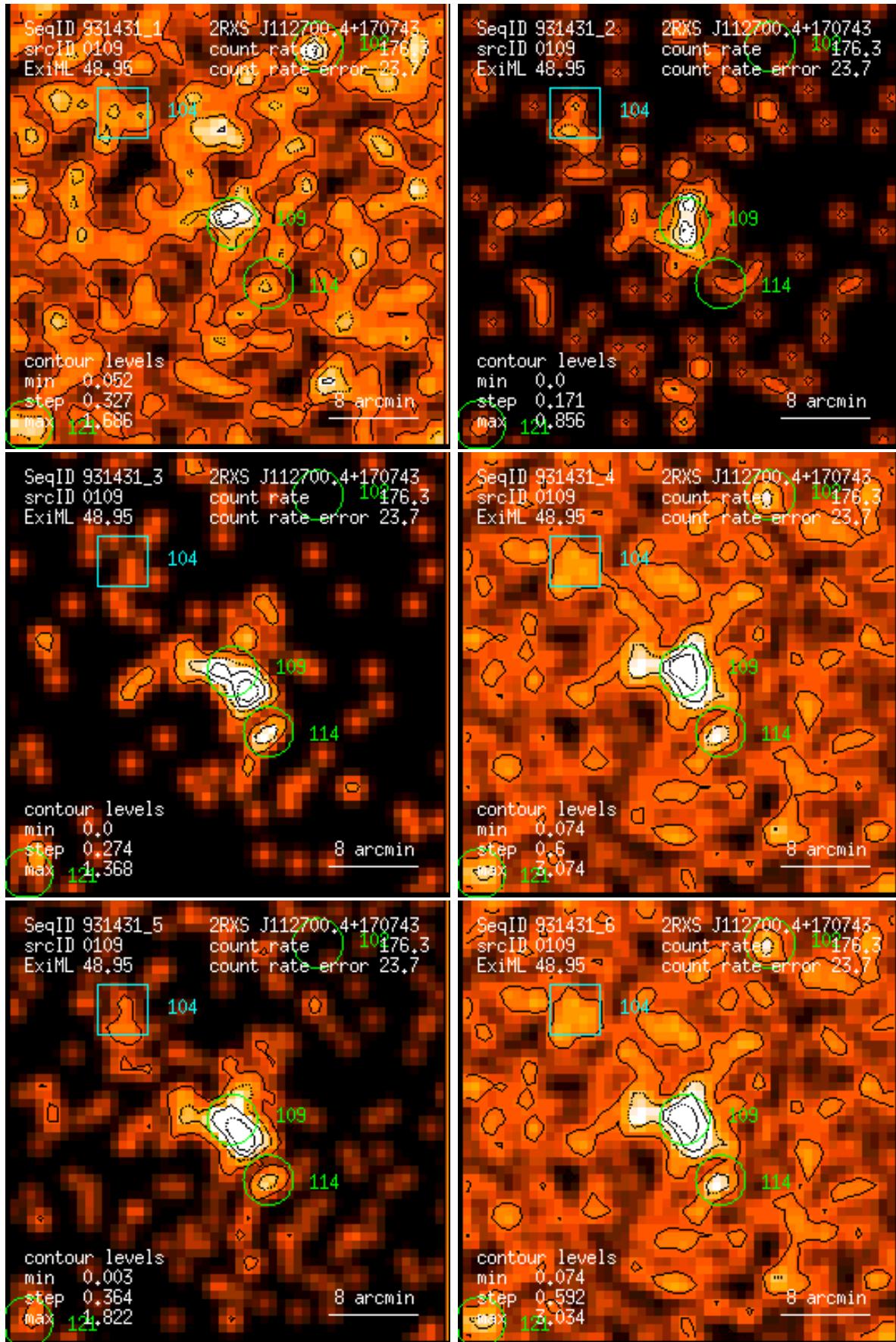
Figure 109: RASS 931431: detection 0109: band rate images, Gaussian filter: (1) PSPC channels 11 – 41, (2) 52 – 90, (3) 91 – 201, (4) 11 – 235, (5) 52 – 201, (6) 11 – 201. Broad band rates in counts/ks. Band rate contour levels in counts/ks/arcmin 2 .
