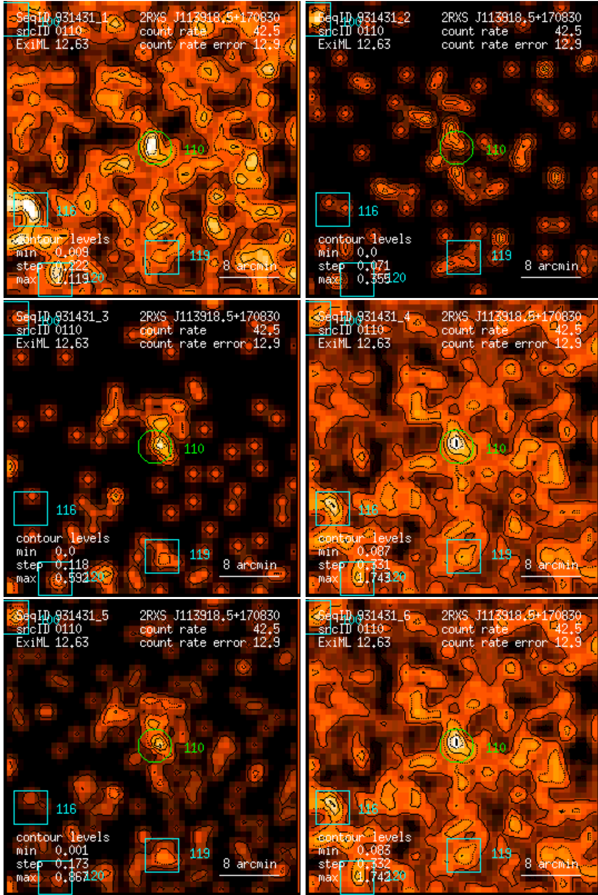
Figure 110: RASS 931431: detection 0110: band rate images, Gaussian filter: (1) PSPC channels 11 – 41, (2) 52 – 90, (3) 91 – 201, (4) 11 – 235, (5) 52 – 201, (6) 11 – 201. Broad band rates in counts/ks. Band rate contour levels in counts/ks/arcmin 2 .
