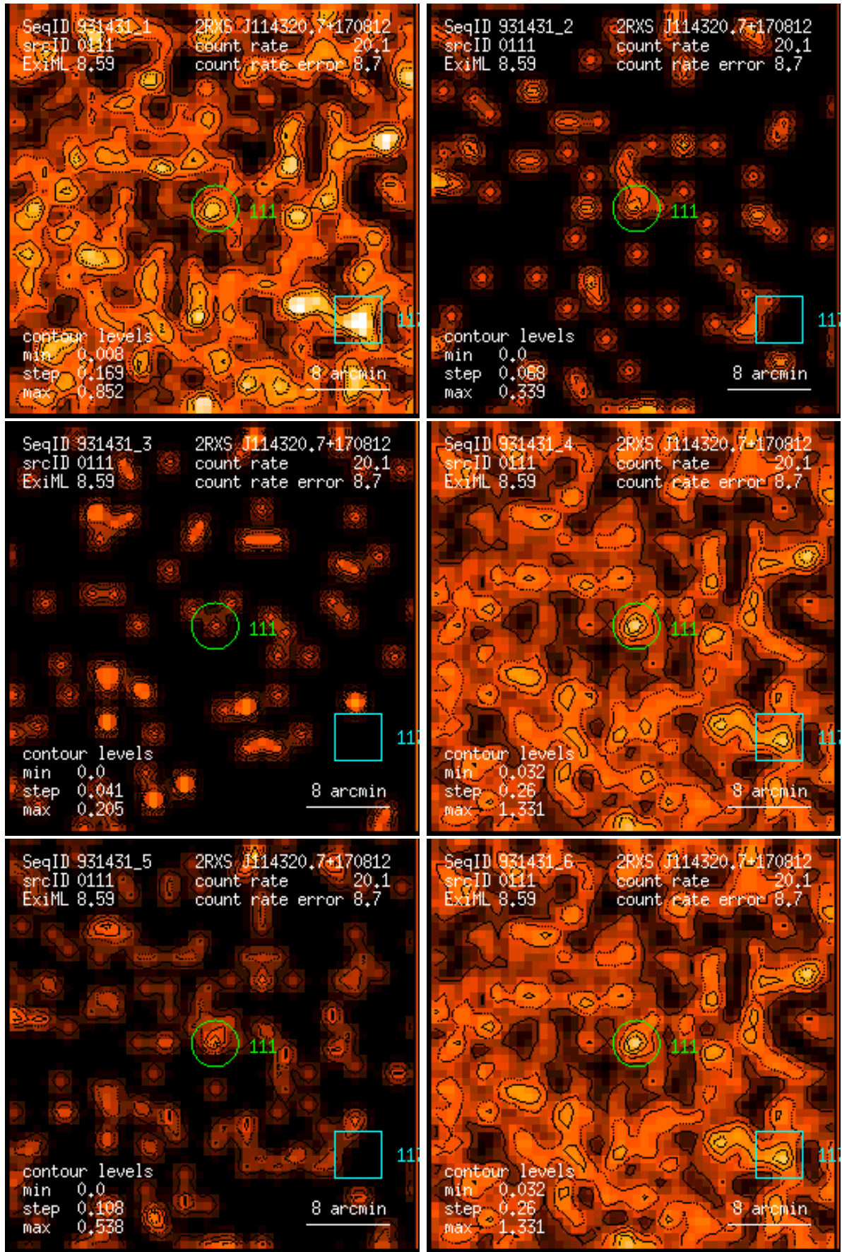
Figure 111: RASS 931431: detection 0111: band rate images, Gaussian filter: (1) PSPC channels 11 – 41, (2) 52 – 90, (3) 91 – 201, (4) 11 – 235, (5) 52 – 201, (6) 11 – 201. Broad band rates in counts/ks. Band rate contour levels in counts/ks/arcmin 2 .
