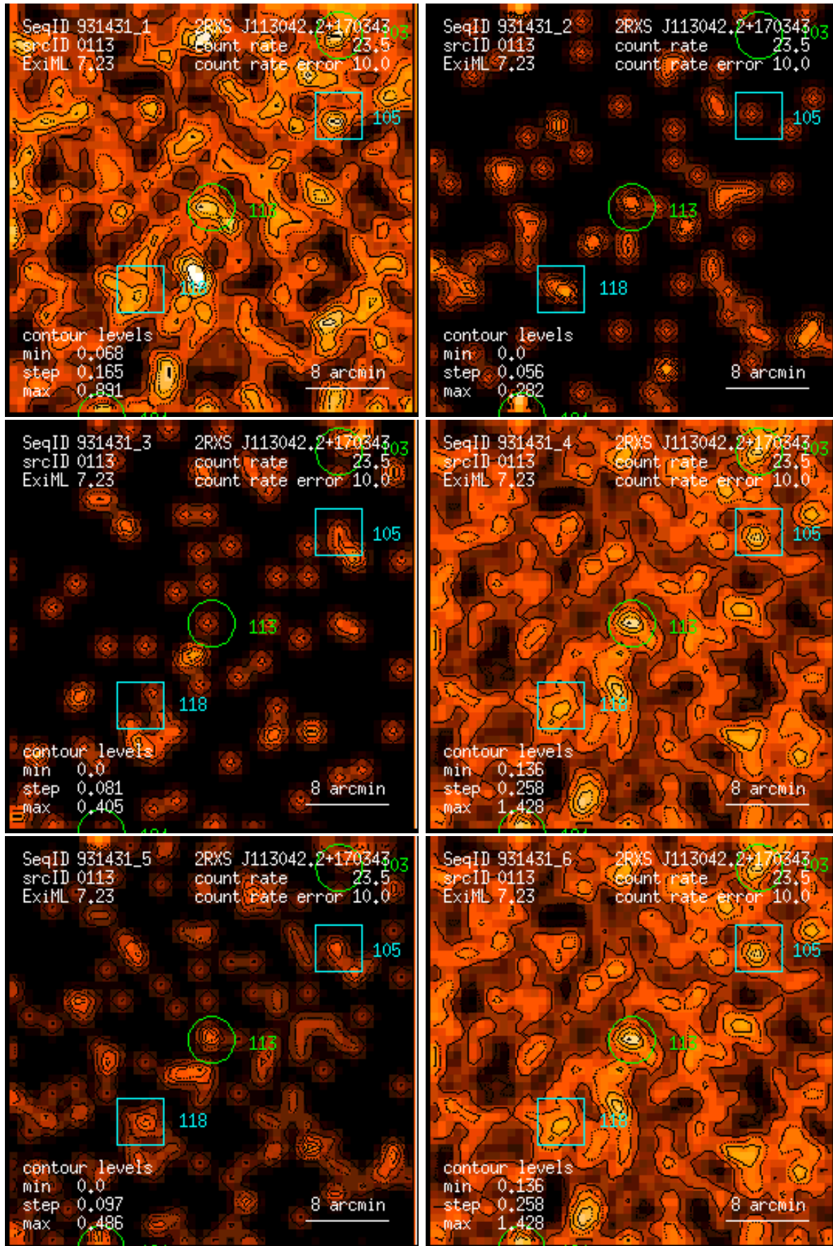
Figure 113: RASS 931431: detection 0113: band rate images, Gaussian filter: (1) PSPC channels 11 – 41, (2) 52 – 90, (3) 91 – 201, (4) 11 – 235, (5) 52 – 201, (6) 11 – 201. Broad band rates in counts/ks. Band rate contour levels in counts/ks/arcmin 2 .
