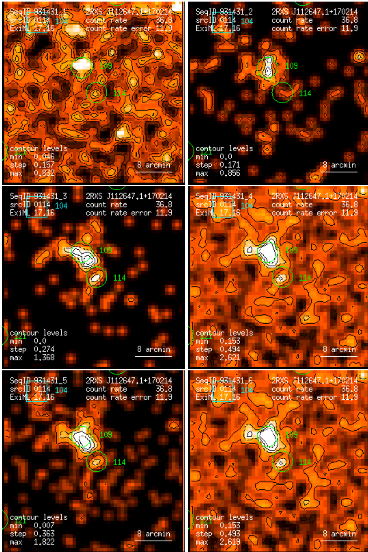
Figure 114: RASS 931431: detection 0114: band rate images, Gaussian filter: (1) PSPC channels 11 – 41, (2) 52 – 90, (3) 91 – 201, (4) 11 – 235, (5) 52 – 201, (6) 11 – 201. Broad band rates in counts/ks. Band rate contour levels in counts/ks/arcmin 2 .
