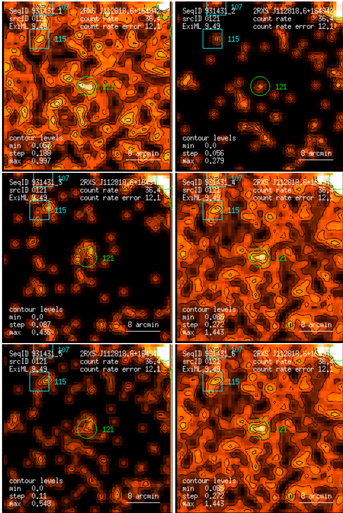
Figure 121: RASS 931431: detection 0121: band rate images, Gaussian filter: (1) PSPC channels 11 – 41, (2) 52 – 90, (3) 91 – 201, (4) 11 – 235, (5) 52 – 201, (6) 11 – 201. Broad band rates in counts/ks. Band rate contour levels in counts/ks/arcmin 2 .
