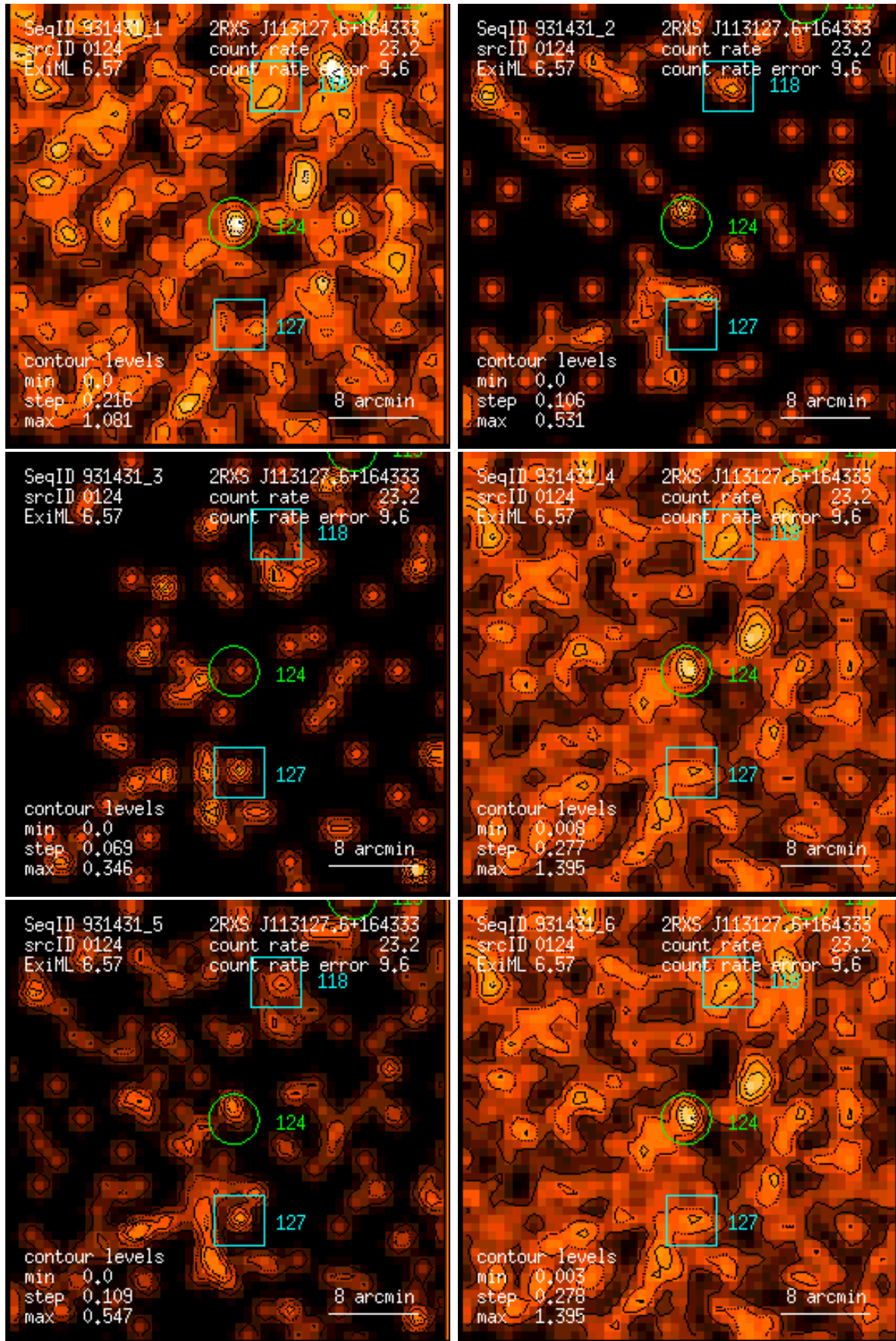
Figure 124: RASS 931431: detection 0124: band rate images, Gaussian filter: (1) PSPC channels 11 – 41, (2) 52 – 90, (3) 91 – 201, (4) 11 – 235, (5) 52 – 201, (6) 11 – 201. Broad band rates in counts/ks. Band rate contour levels in counts/ks/arcmin 2 .
