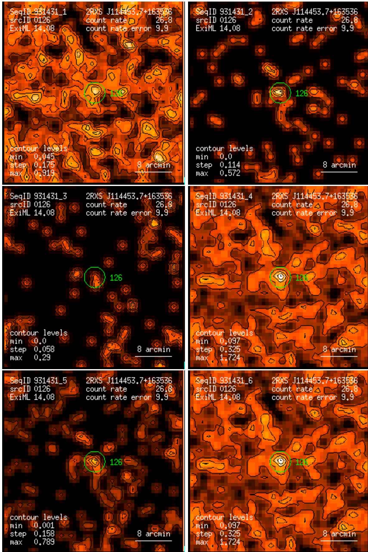
Figure 126: RASS 931431: detection 0126: band rate images, Gaussian filter: (1) PSPC channels 11 – 41, (2) 52 – 90, (3) 91 – 201, (4) 11 – 235, (5) 52 – 201, (6) 11 – 201. Broad band rates in counts/ks. Band rate contour levels in counts/ks/arcmin 2 .
