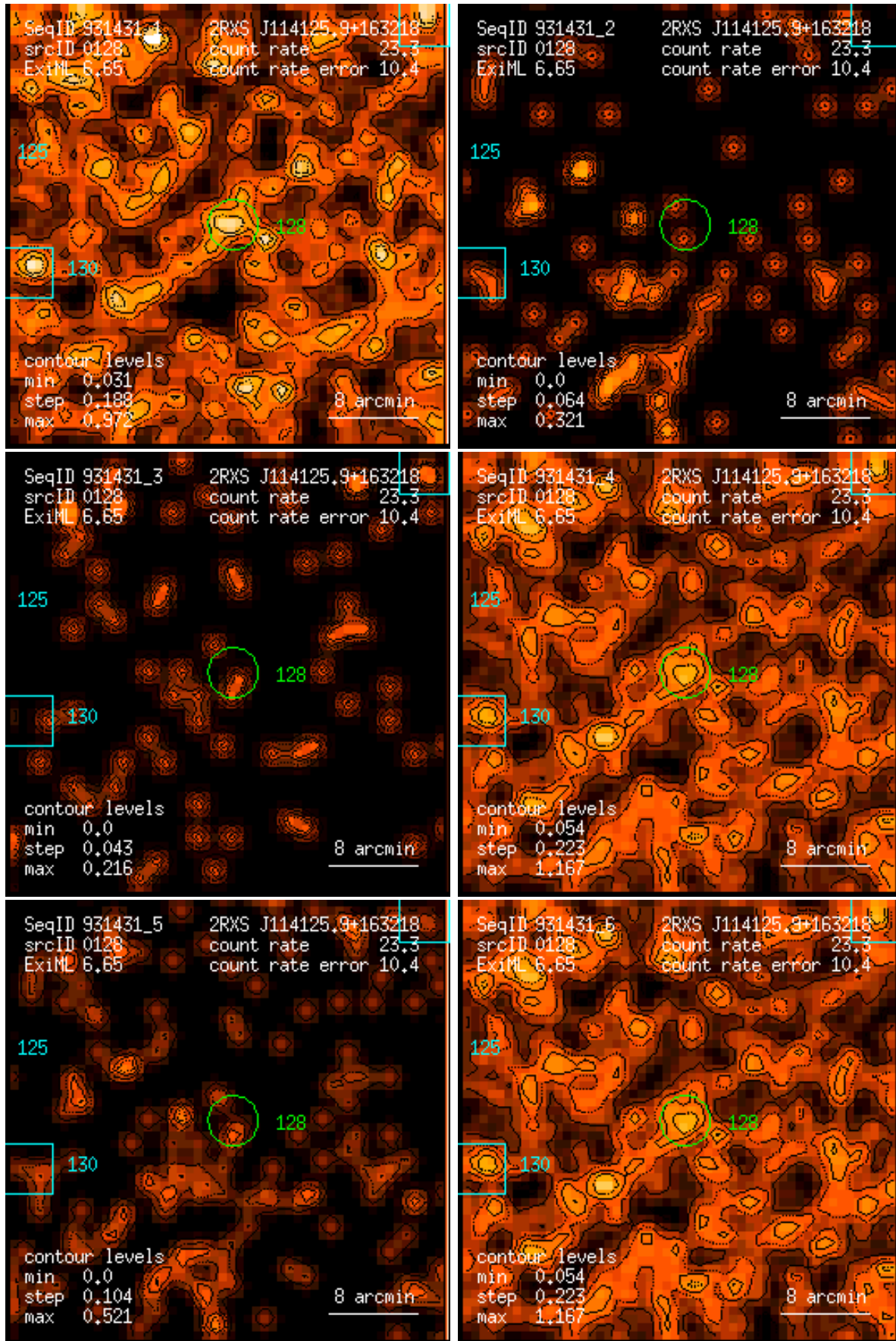
Figure 128: RASS 931431: detection 0128: band rate images, Gaussian filter: (1) PSPC channels 11 – 41, (2) 52 – 90, (3) 91 – 201, (4) 11 – 235, (5) 52 – 201, (6) 11 – 201. Broad band rates in counts/ks. Band rate contour levels in counts/ks/arcmin 2 .
