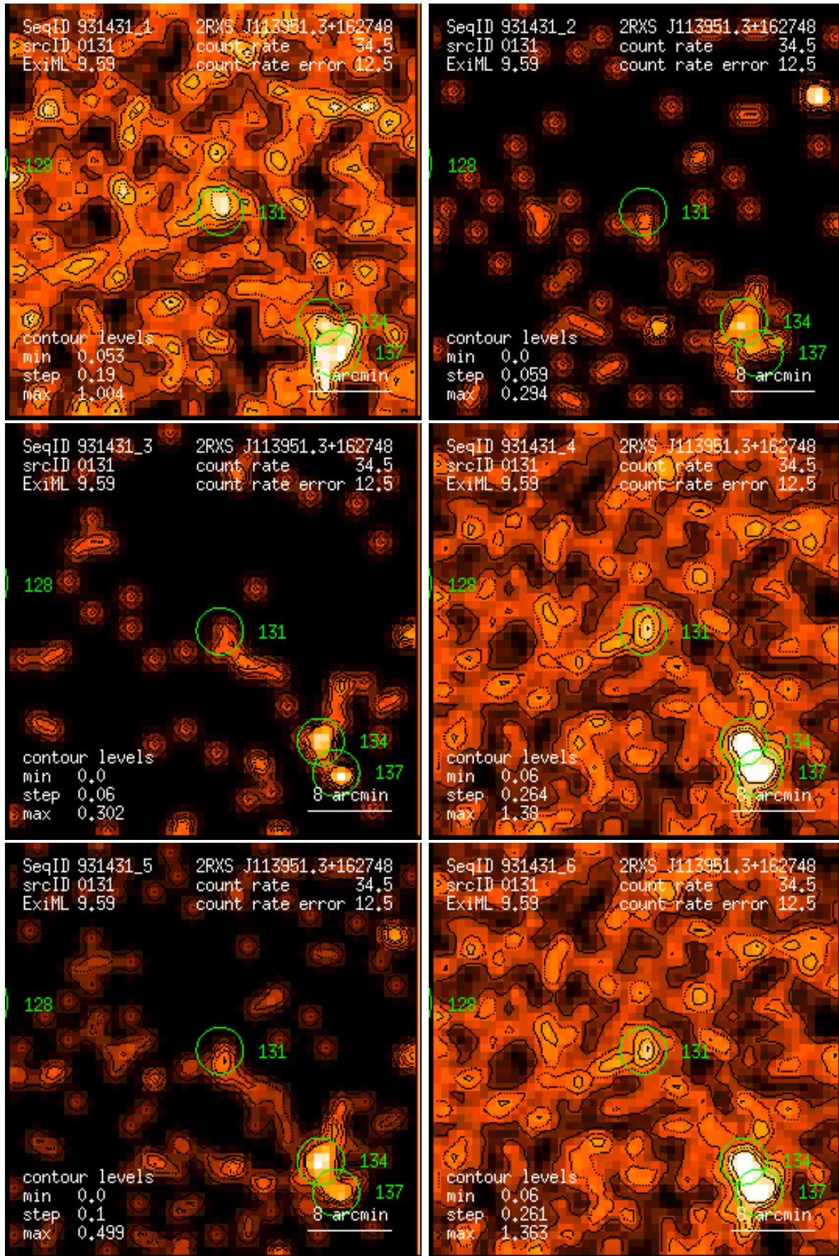
Figure 131: RASS 931431: detection 0131: band rate images, Gaussian filter: (1) PSPC channels 11 – 41, (2) 52 – 90, (3) 91 – 201, (4) 11 – 235, (5) 52 – 201, (6) 11 – 201. Broad band rates in counts/ks. Band rate contour levels in counts/ks/arcmin 2 .
