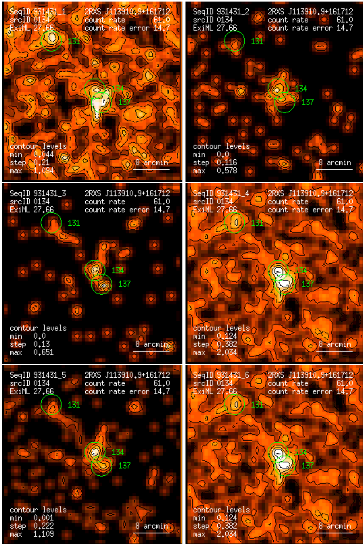
Figure 134: RASS 931431: detection 0134: band rate images, Gaussian filter: (1) PSPC channels 11 – 41, (2) 52 – 90, (3) 91 – 201, (4) 11 – 235, (5) 52 – 201, (6) 11 – 201. Broad band rates in counts/ks. Band rate contour levels in counts/ks/arcmin 2 .
