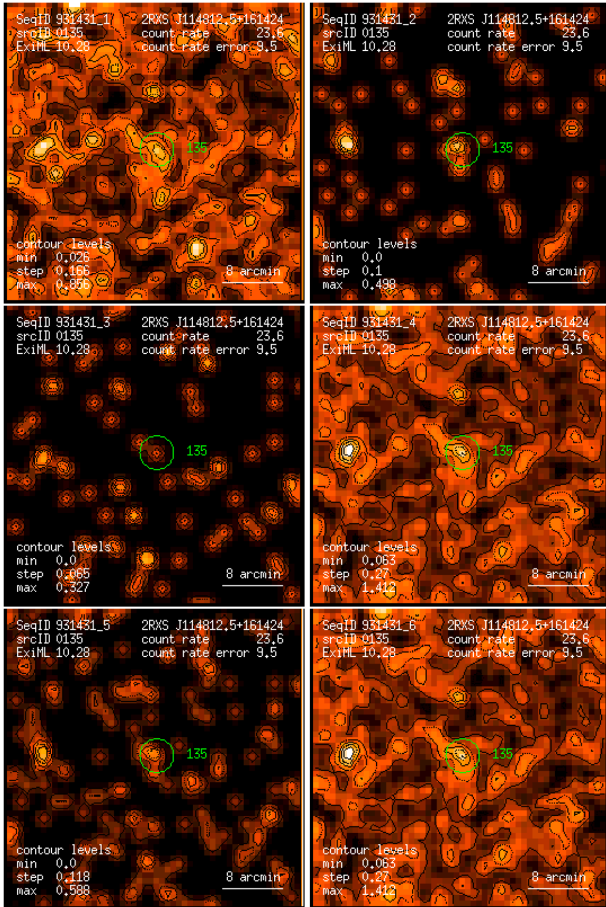
Figure 135: RASS 931431: detection 0135: band rate images, Gaussian filter: (1) PSPC channels 11 – 41, (2) 52 – 90, (3) 91 – 201, (4) 11 – 235, (5) 52 – 201, (6) 11 – 201. Broad band rates in counts/ks. Band rate contour levels in counts/ks/arcmin 2 .
