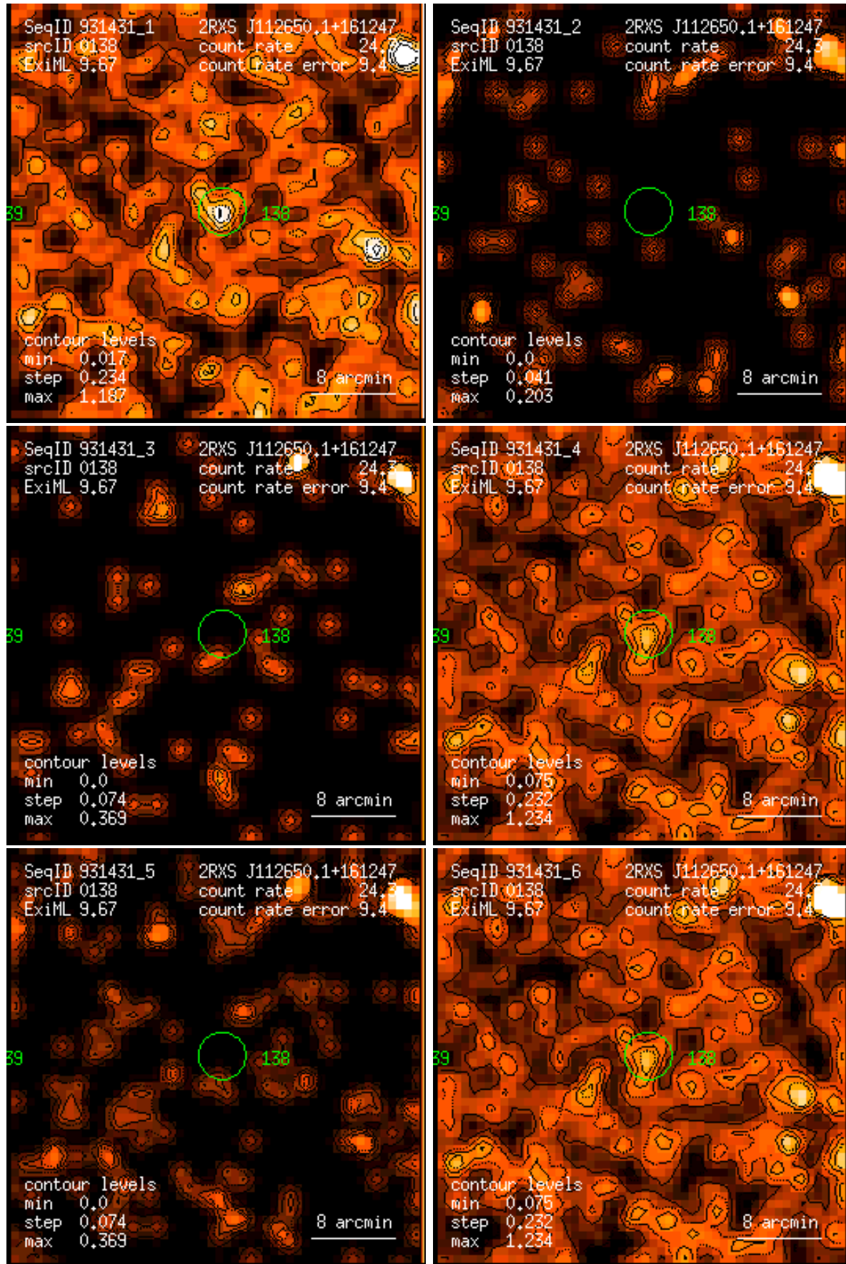
Figure 138: RASS 931431: detection 0138: band rate images, Gaussian filter: (1) PSPC channels 11 – 41, (2) 52 – 90, (3) 91 – 201, (4) 11 – 235, (5) 52 – 201, (6) 11 – 201. Broad band rates in counts/ks. Band rate contour levels in counts/ks/arcmin 2 .
