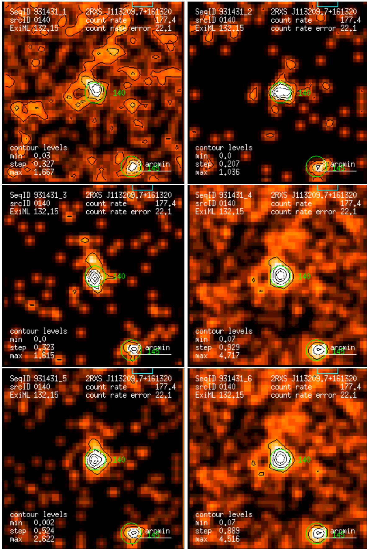
Figure 140: RASS 931431: detection 0140: band rate images, Gaussian filter: (1) PSPC channels 11 – 41, (2) 52 – 90, (3) 91 – 201, (4) 11 – 235, (5) 52 – 201, (6) 11 – 201. Broad band rates in counts/ks. Band rate contour levels in counts/ks/arcmin 2 .
