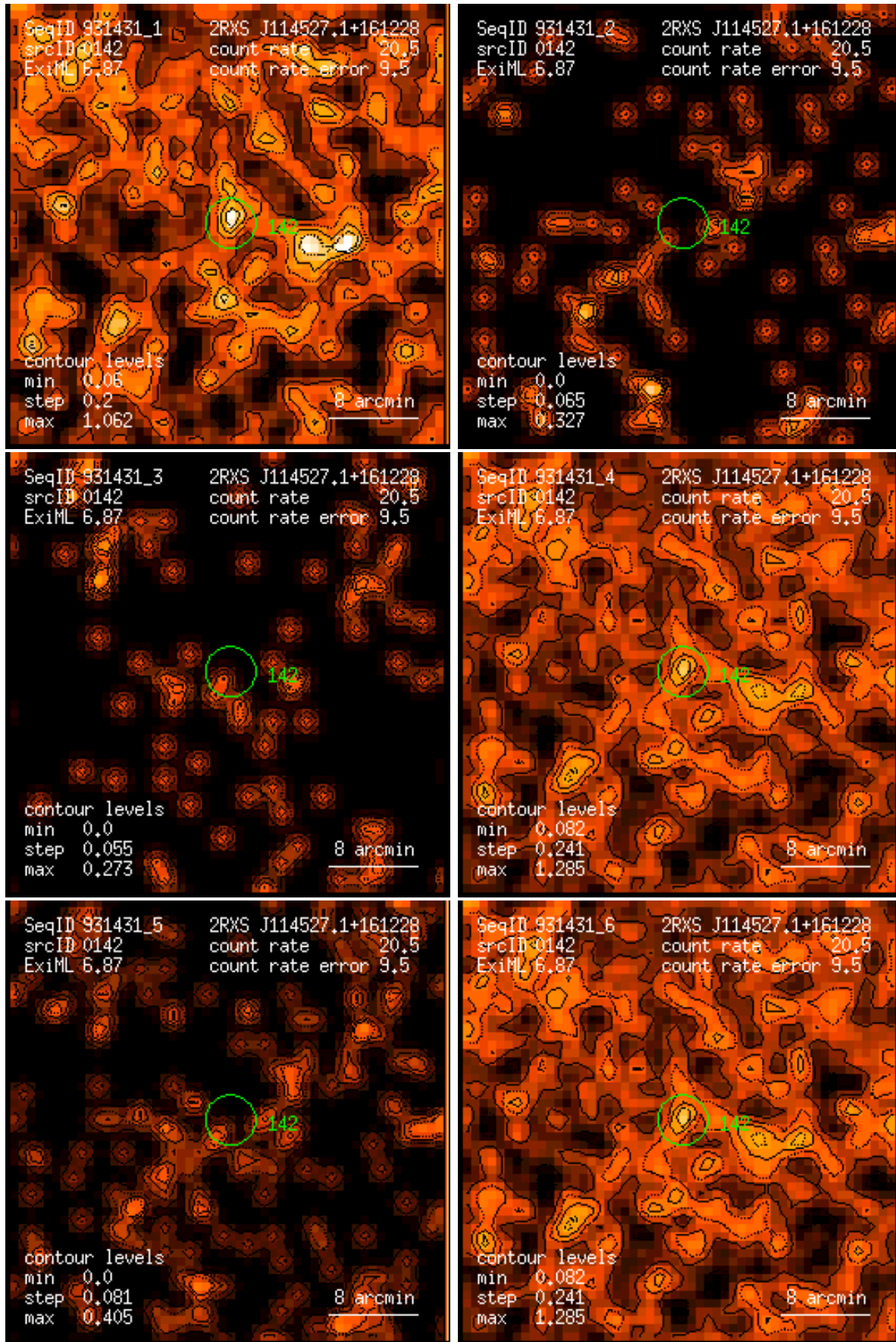
Figure 142: RASS 931431: detection 0142: band rate images, Gaussian filter: (1) PSPC channels 11 – 41, (2) 52 – 90, (3) 91 – 201, (4) 11 – 235, (5) 52 – 201, (6) 11 – 201. Broad band rates in counts/ks. Band rate contour levels in counts/ks/arcmin 2 .
