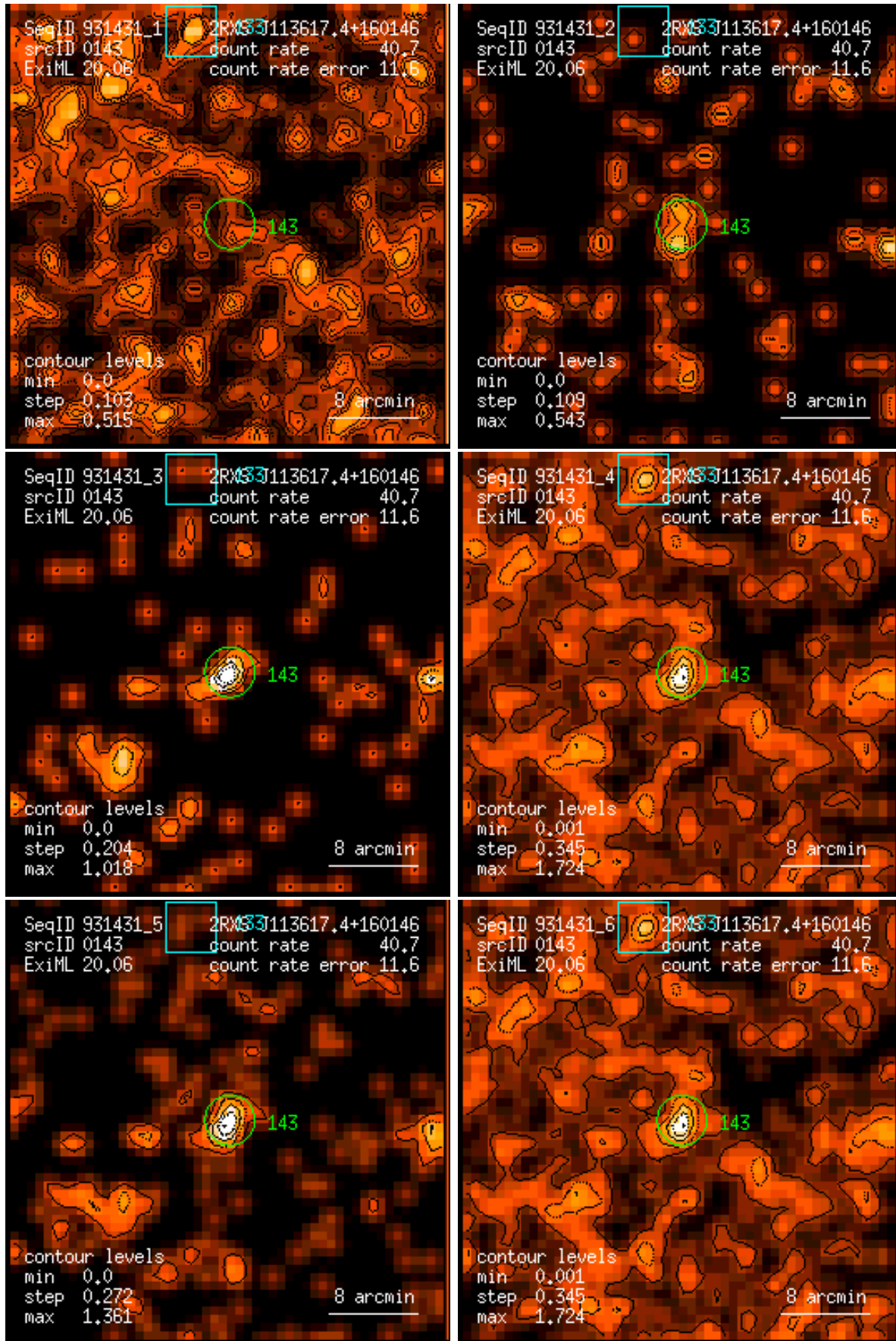
Figure 143: RASS 931431: detection 0143: band rate images, Gaussian filter: (1) PSPC channels 11 – 41, (2) 52 – 90, (3) 91 – 201, (4) 11 – 235, (5) 52 – 201, (6) 11 – 201. Broad band rates in counts/ks. Band rate contour levels in counts/ks/arcmin 2 .
