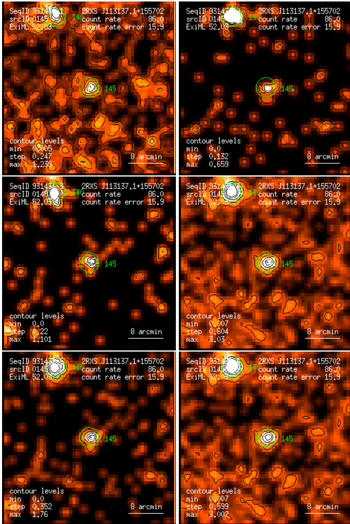
Figure 145: RASS 931431: detection 0145: band rate images, Gaussian filter: (1) PSPC channels 11 – 41, (2) 52 – 90, (3) 91 – 201, (4) 11 – 235, (5) 52 – 201, (6) 11 – 201. Broad band rates in counts/ks. Band rate contour levels in counts/ks/arcmin 2 .
