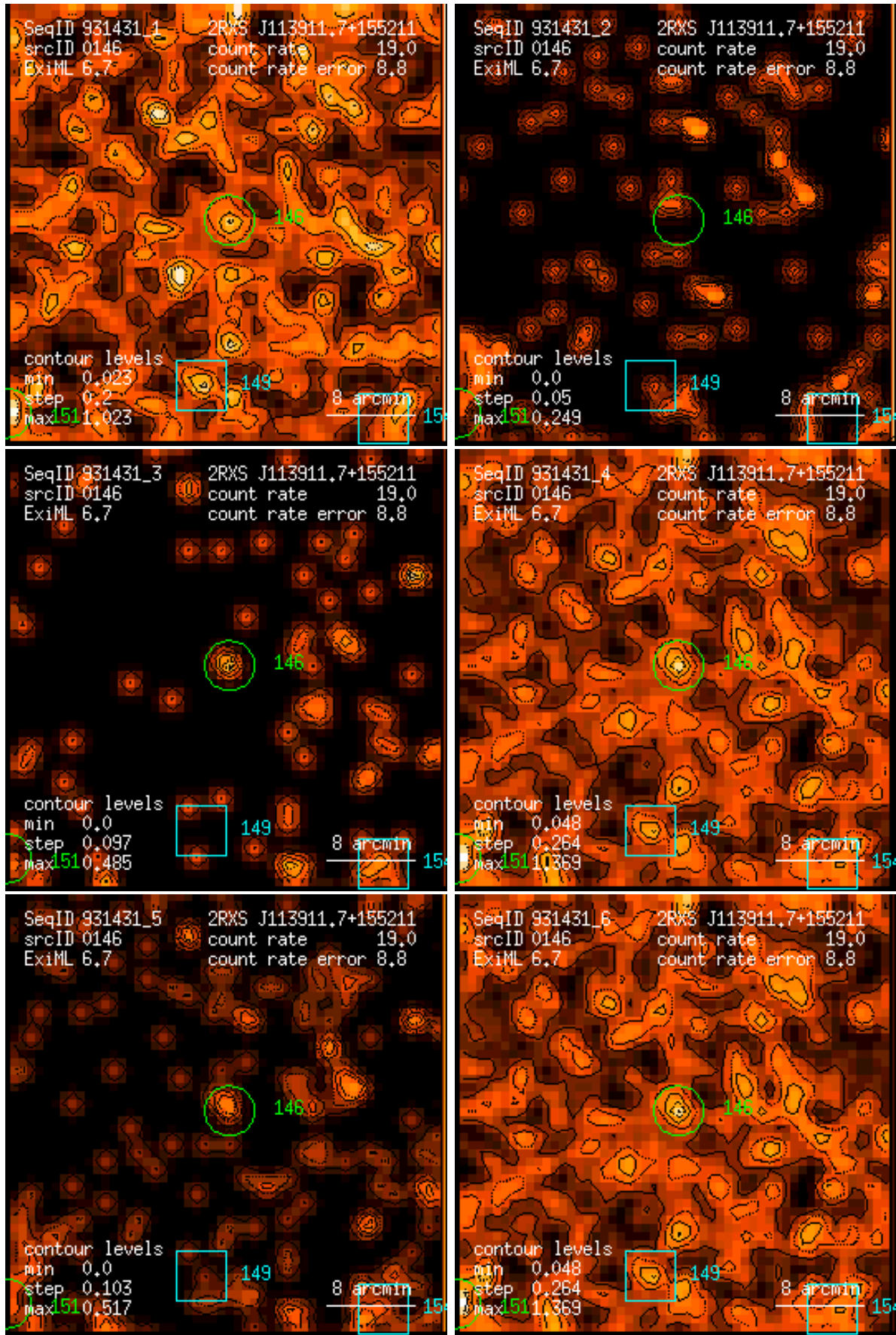
Figure 146: RASS 931431: detection 0146: band rate images, Gaussian filter: (1) PSPC channels 11 – 41, (2) 52 – 90, (3) 91 – 201, (4) 11 – 235, (5) 52 – 201, (6) 11 – 201. Broad band rates in counts/ks. Band rate contour levels in counts/ks/arcmin 2 .
