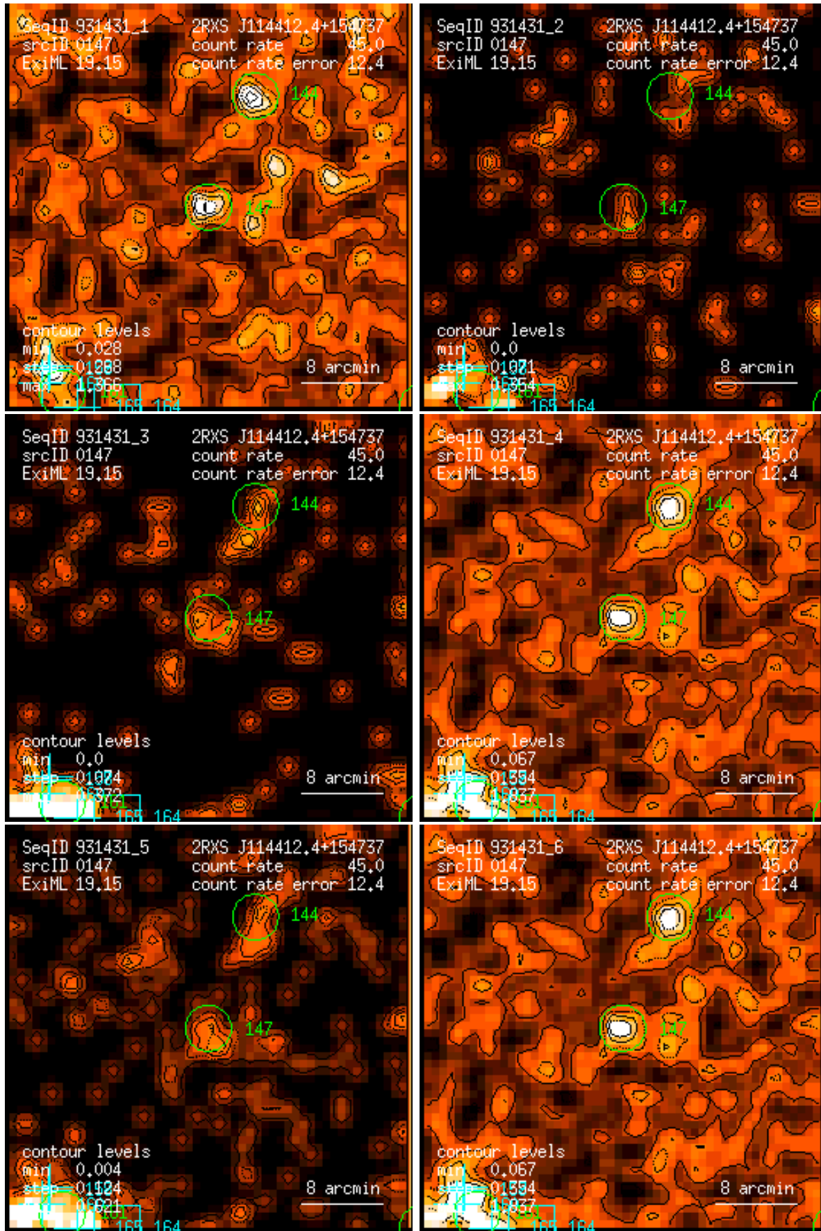
Figure 147: RASS 931431: detection 0147: band rate images, Gaussian filter: (1) PSPC channels 11 – 41, (2) 52 – 90, (3) 91 – 201, (4) 11 – 235, (5) 52 – 201, (6) 11 – 201. Broad band rates in counts/ks. Band rate contour levels in counts/ks/arcmin 2 .
