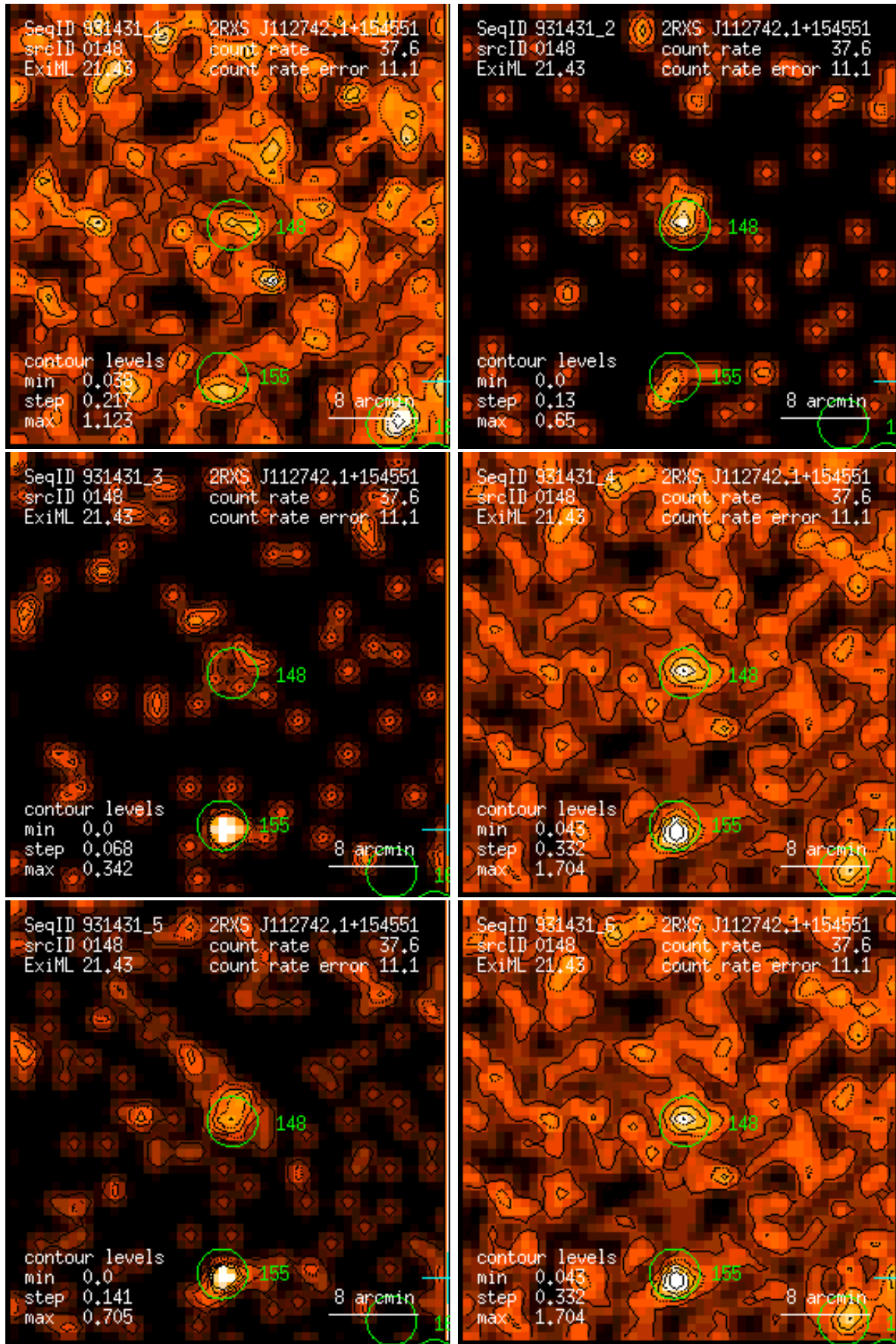
Figure 148: RASS 931431: detection 0148: band rate images, Gaussian filter: (1) PSPC channels 11 – 41, (2) 52 – 90, (3) 91 – 201, (4) 11 – 235, (5) 52 – 201, (6) 11 – 201. Broad band rates in counts/ks. Band rate contour levels in counts/ks/arcmin 2 .
