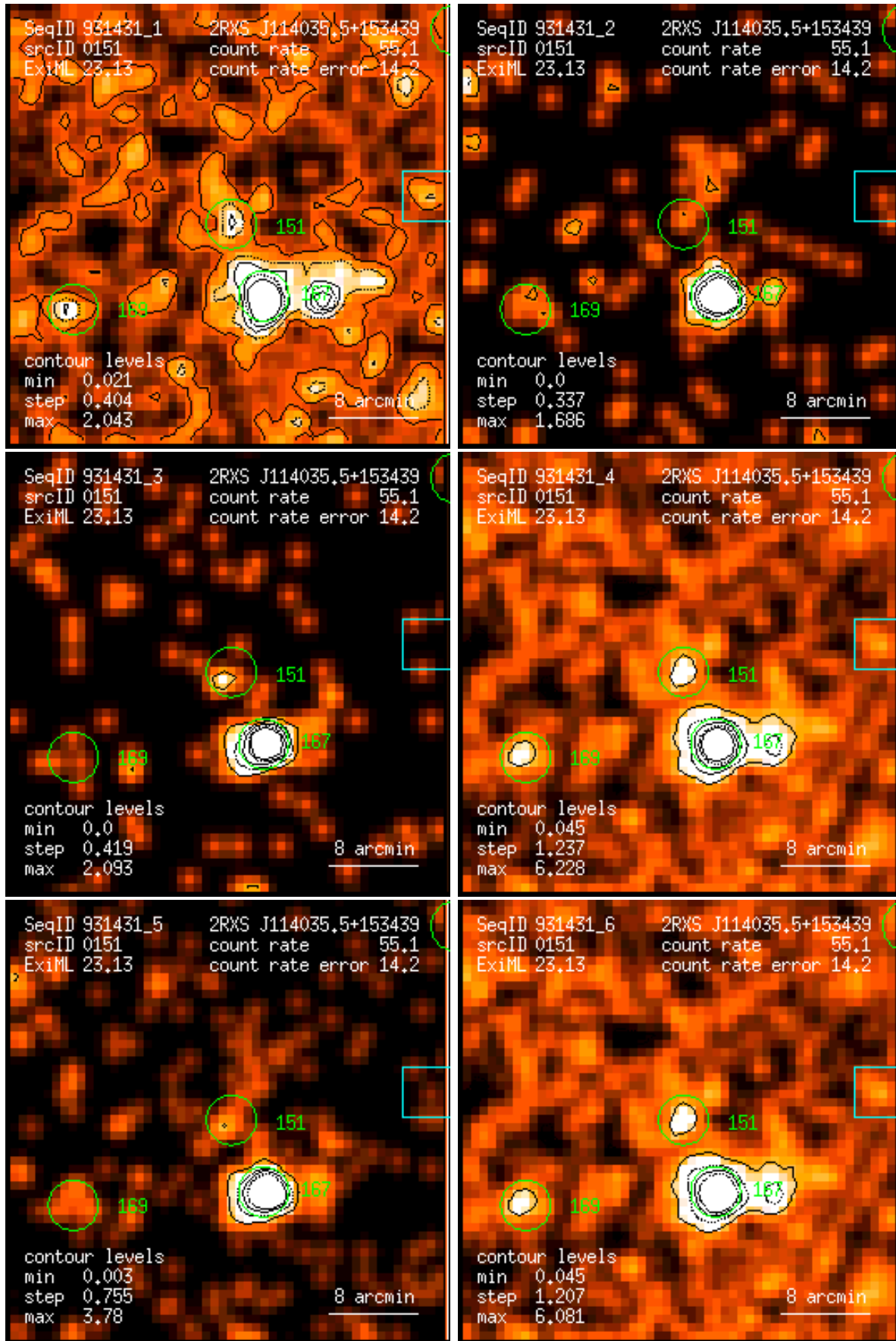
Figure 151: RASS 931431: detection 0151: band rate images, Gaussian filter: (1) PSPC channels 11 – 41, (2) 52 – 90, (3) 91 – 201, (4) 11 – 235, (5) 52 – 201, (6) 11 – 201. Broad band rates in counts/ks. Band rate contour levels in counts/ks/arcmin 2 .
