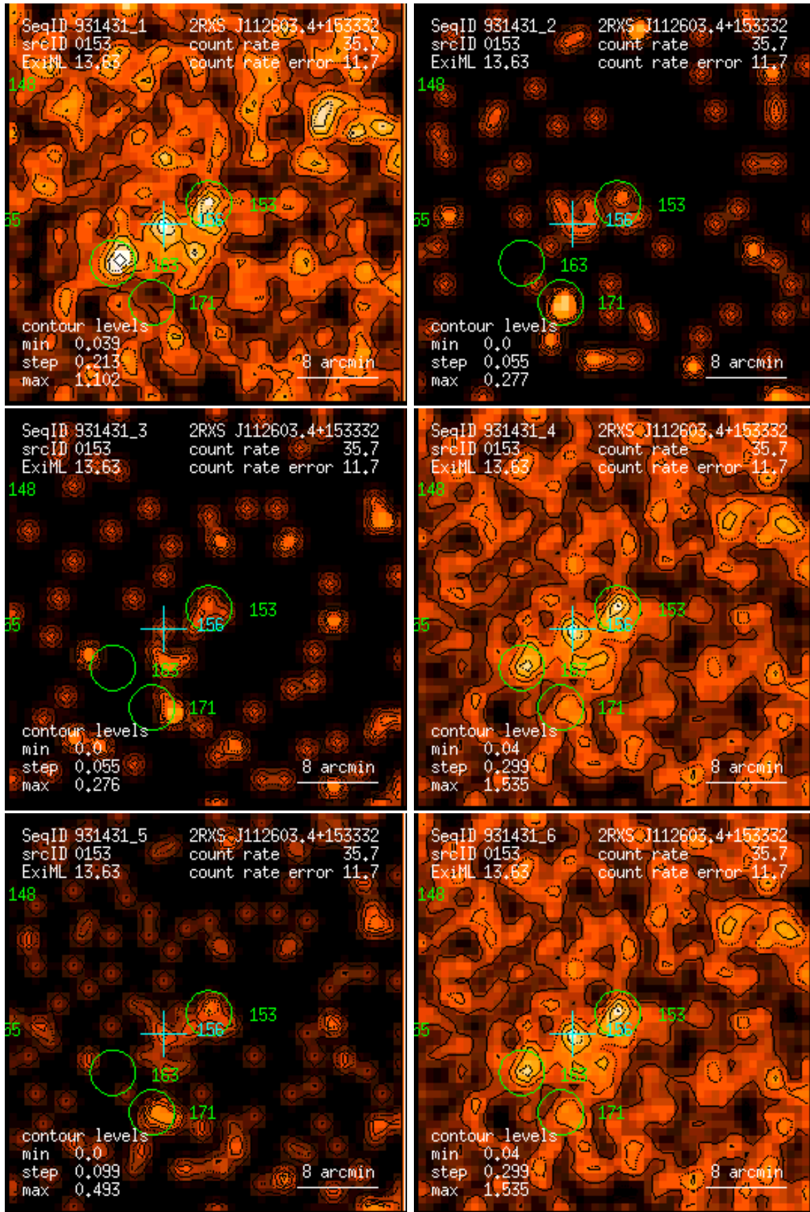
Figure 153: RASS 931431: detection 0153: band rate images, Gaussian filter: (1) PSPC channels 11 – 41, (2) 52 – 90, (3) 91 – 201, (4) 11 – 235, (5) 52 – 201, (6) 11 – 201. Broad band rates in counts/ks. Band rate contour levels in counts/ks/arcmin 2 .
