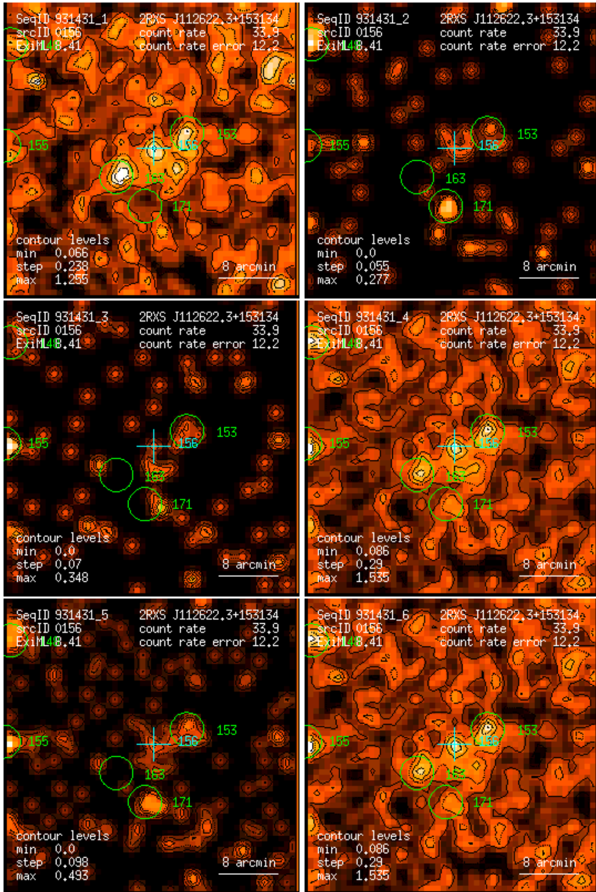
Figure 156: RASS 931431: detection 0156: band rate images, Gaussian filter: (1) PSPC channels 11 – 41, (2) 52 – 90, (3) 91 – 201, (4) 11 – 235, (5) 52 – 201, (6) 11 – 201. Broad band rates in counts/ks. Band rate contour levels in counts/ks/arcmin 2 .
