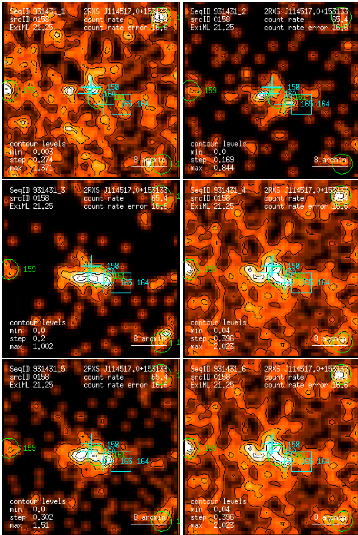
Figure 158: RASS 931431: detection 0158: band rate images, Gaussian filter: (1) PSPC channels 11 – 41, (2) 52 – 90, (3) 91 – 201, (4) 11 – 235, (5) 52 – 201, (6) 11 – 201. Broad band rates in counts/ks. Band rate contour levels in counts/ks/arcmin 2 .
