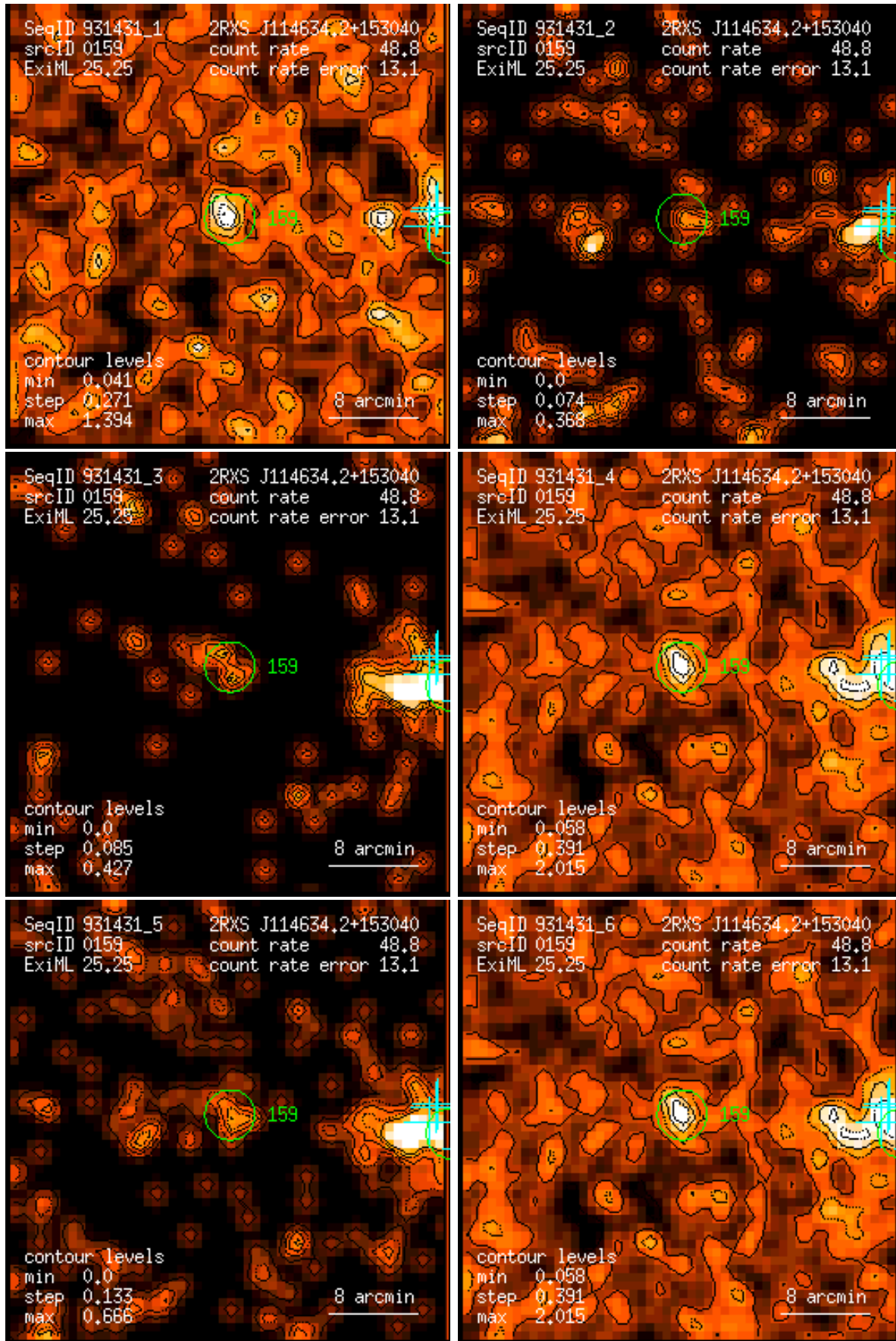
Figure 159: RASS 931431: detection 0159: band rate images, Gaussian filter: (1) PSPC channels 11 – 41, (2) 52 – 90, (3) 91 – 201, (4) 11 – 235, (5) 52 – 201, (6) 11 – 201. Broad band rates in counts/ks. Band rate contour levels in counts/ks/arcmin 2 .
