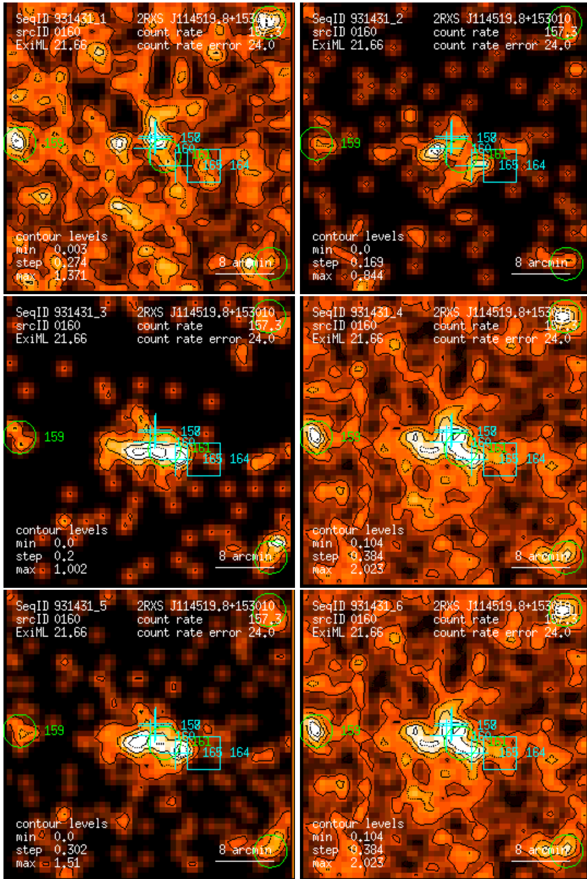
Figure 160: RASS 931431: detection 0160: band rate images, Gaussian filter: (1) PSPC channels 11 – 41, (2) 52 – 90, (3) 91 – 201, (4) 11 – 235, (5) 52 – 201, (6) 11 – 201. Broad band rates in counts/ks. Band rate contour levels in counts/ks/arcmin 2 .
