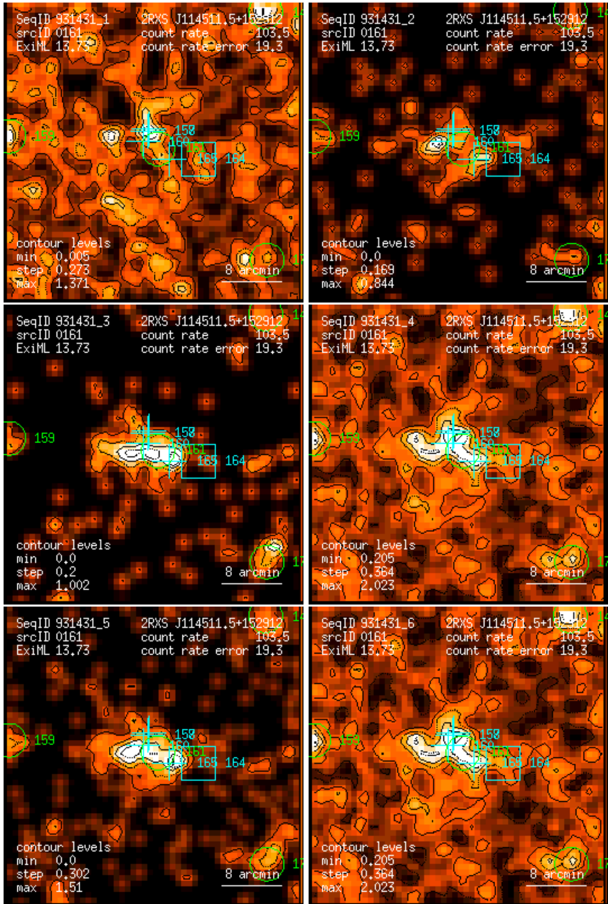
Figure 161: RASS 931431: detection 0161: band rate images, Gaussian filter: (1) PSPC channels 11 – 41, (2) 52 – 90, (3) 91 – 201, (4) 11 – 235, (5) 52 – 201, (6) 11 – 201. Broad band rates in counts/ks. Band rate contour levels in counts/ks/arcmin 2 .
