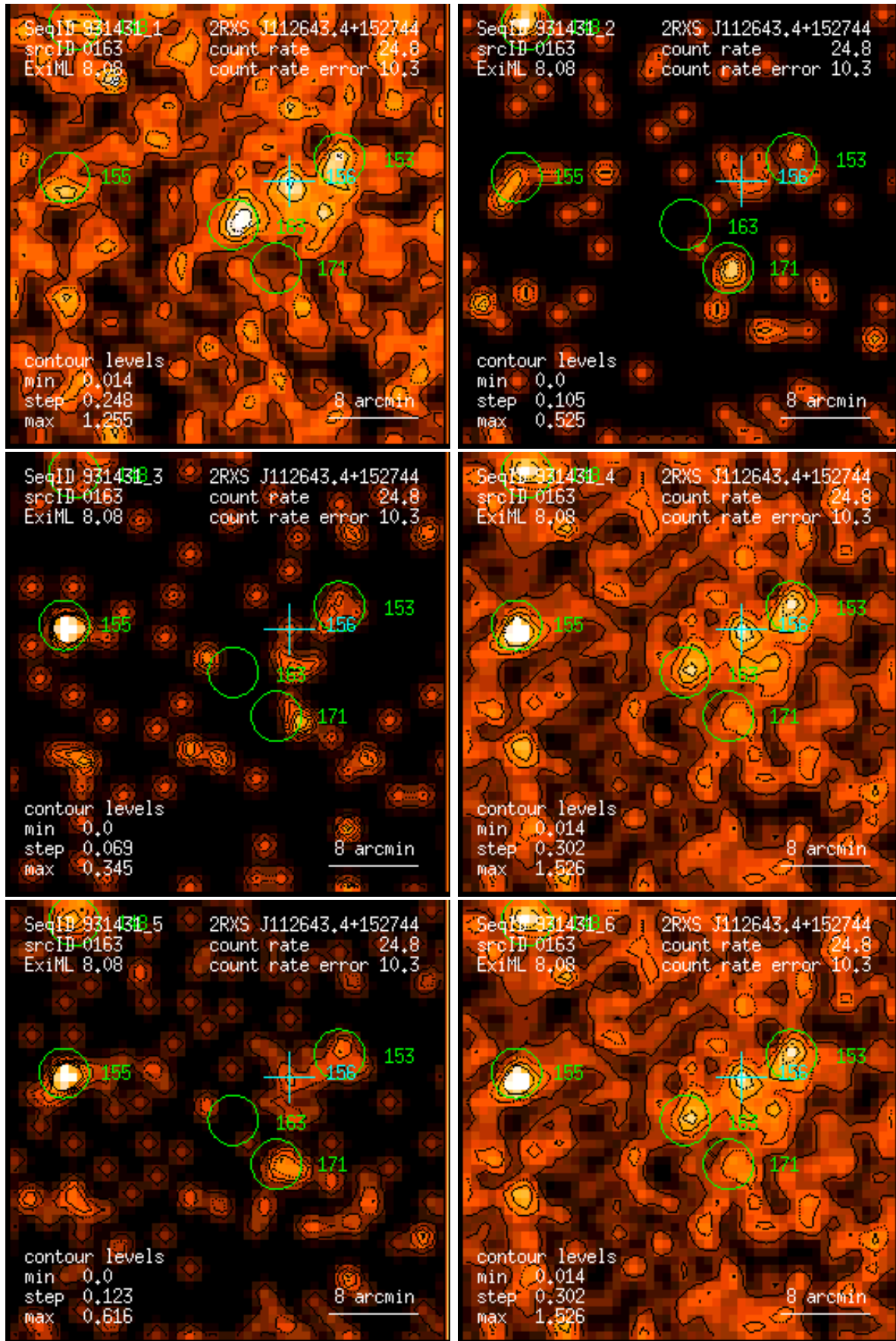
Figure 163: RASS 931431: detection 0163: band rate images, Gaussian filter: (1) PSPC channels 11 – 41, (2) 52 – 90, (3) 91 – 201, (4) 11 – 235, (5) 52 – 201, (6) 11 – 201. Broad band rates in counts/ks. Band rate contour levels in counts/ks/arcmin 2 .
