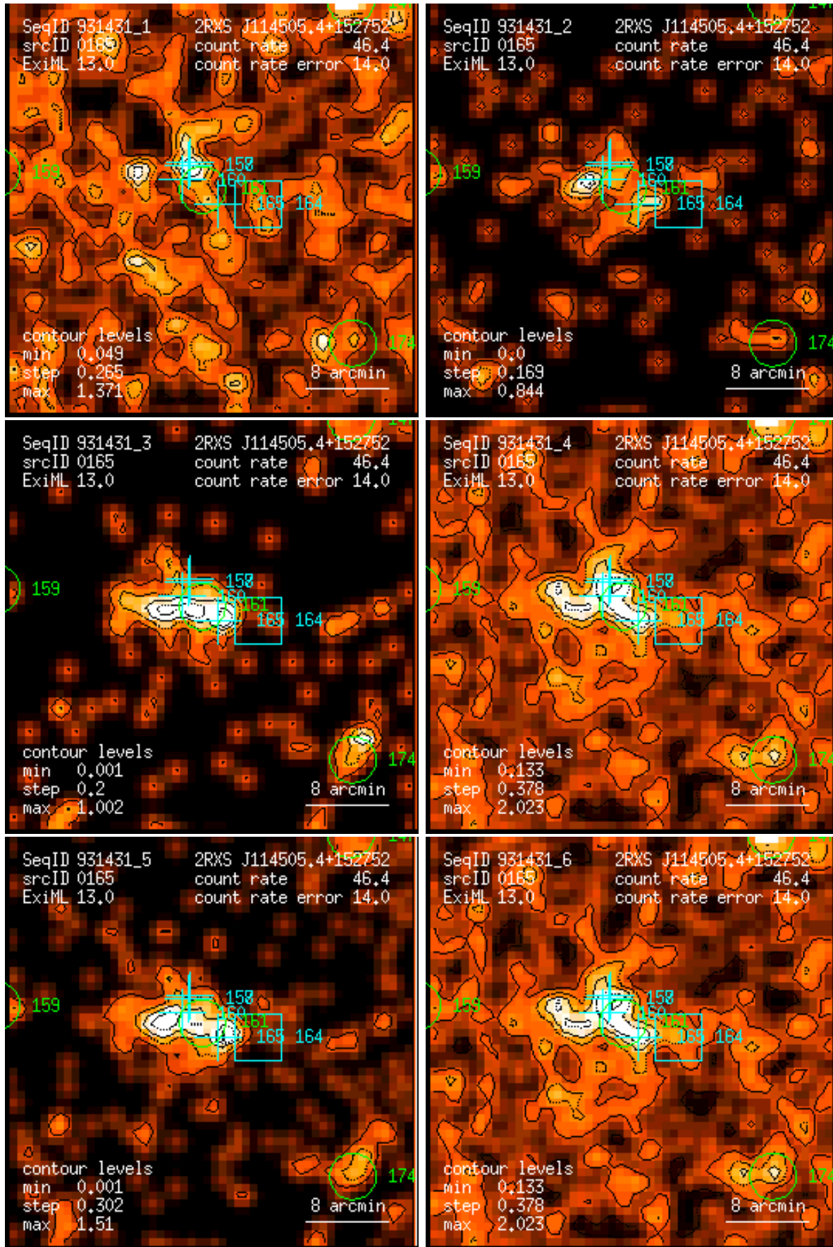
Figure 165: RASS 931431: detection 0165: band rate images, Gaussian filter: (1) PSPC channels 11 – 41, (2) 52 – 90, (3) 91 – 201, (4) 11 – 235, (5) 52 – 201, (6) 11 – 201. Broad band rates in counts/ks. Band rate contour levels in counts/ks/arcmin 2 .
