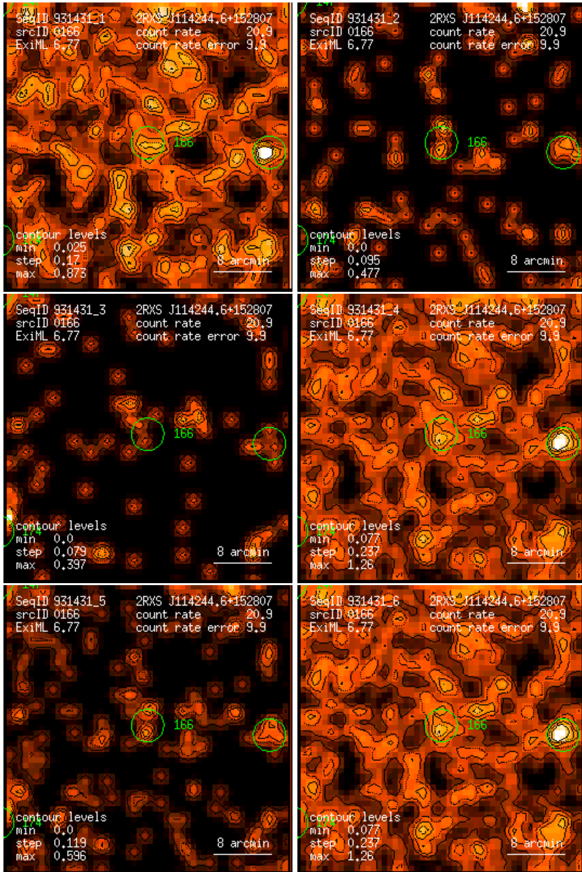
Figure 166: RASS 931431: detection 0166: band rate images, Gaussian filter: (1) PSPC channels 11 – 41, (2) 52 – 90, (3) 91 – 201, (4) 11 – 235, (5) 52 – 201, (6) 11 – 201. Broad band rates in counts/ks. Band rate contour levels in counts/ks/arcmin 2 .
