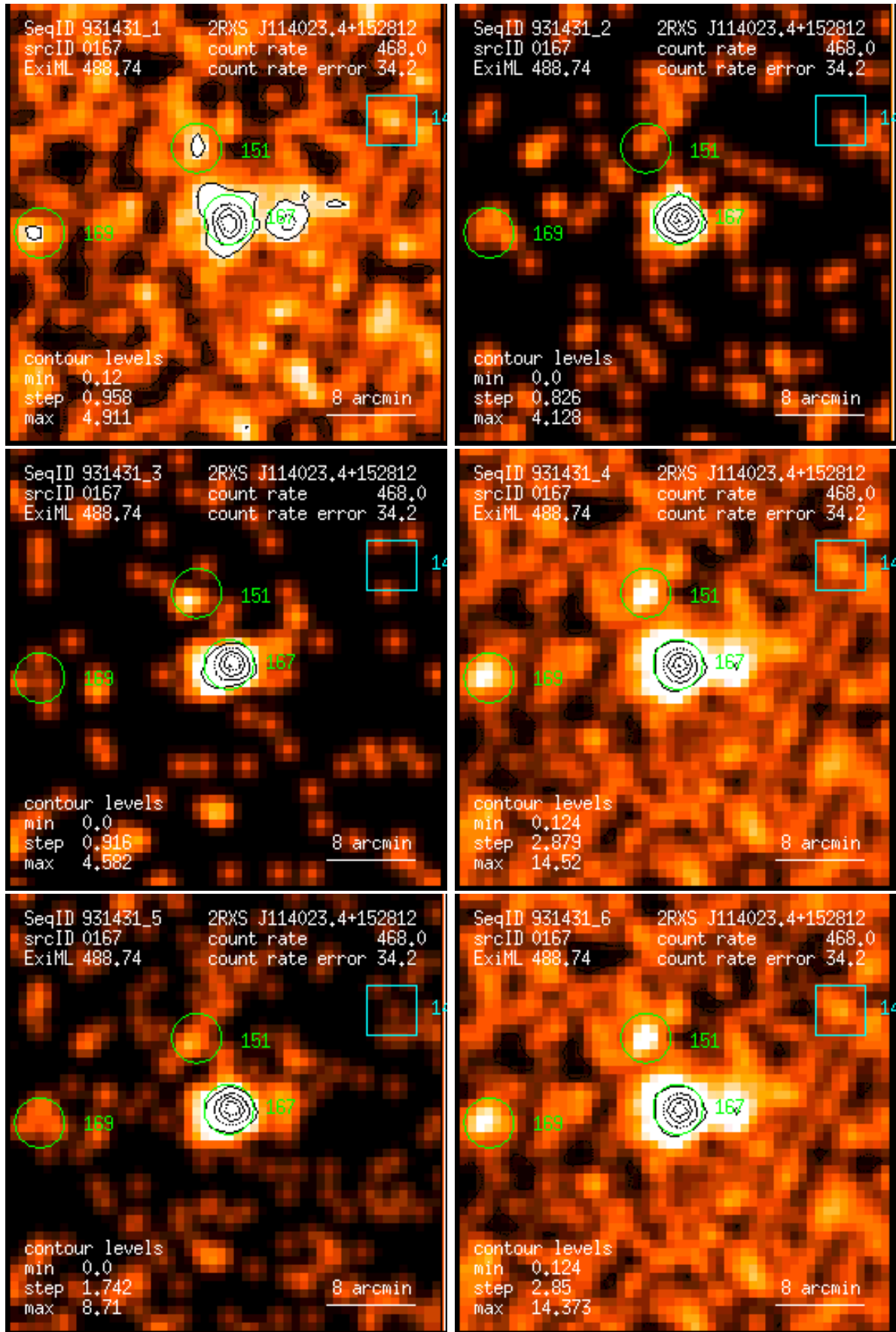
Figure 167: RASS 931431: detection 0167: band rate images, Gaussian filter: (1) PSPC channels 11 – 41, (2) 52 – 90, (3) 91 – 201, (4) 11 – 235, (5) 52 – 201, (6) 11 – 201. Broad band rates in counts/ks. Band rate contour levels in counts/ks/arcmin 2 .
