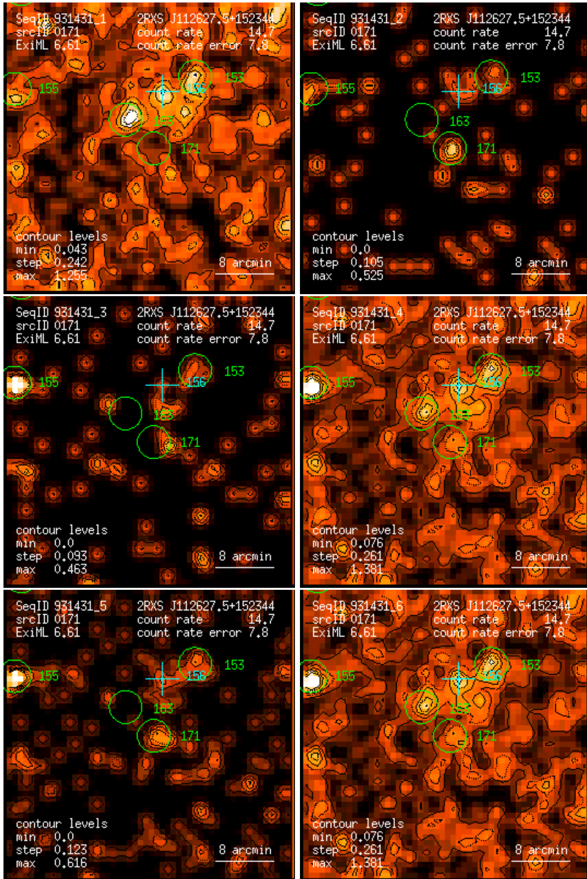
Figure 171: RASS 931431: detection 0171: band rate images, Gaussian filter: (1) PSPC channels 11 – 41, (2) 52 – 90, (3) 91 – 201, (4) 11 – 235, (5) 52 – 201, (6) 11 – 201. Broad band rates in counts/ks. Band rate contour levels in counts/ks/arcmin 2 .
