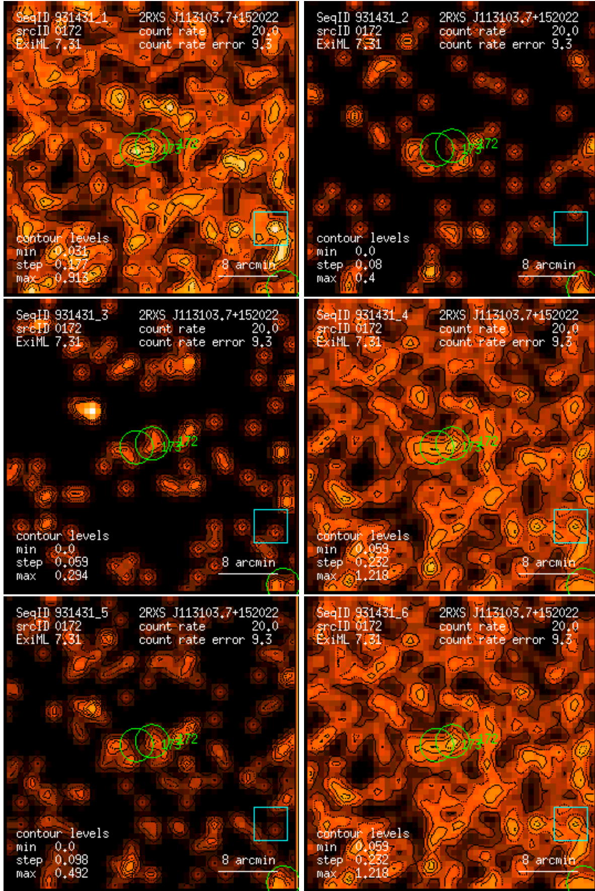
Figure 172: RASS 931431: detection 0172: band rate images, Gaussian filter: (1) PSPC channels 11 – 41, (2) 52 – 90, (3) 91 – 201, (4) 11 – 235, (5) 52 – 201, (6) 11 – 201. Broad band rates in counts/ks. Band rate contour levels in counts/ks/arcmin 2 .
