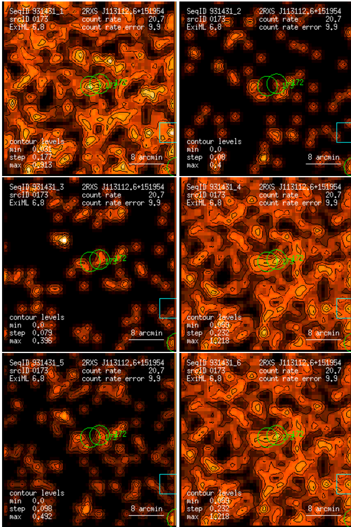
Figure 173: RASS 931431: detection 0173: band rate images, Gaussian filter: (1) PSPC channels 11 – 41, (2) 52 – 90, (3) 91 – 201, (4) 11 – 235, (5) 52 – 201, (6) 11 – 201. Broad band rates in counts/ks. Band rate contour levels in counts/ks/arcmin 2 .
