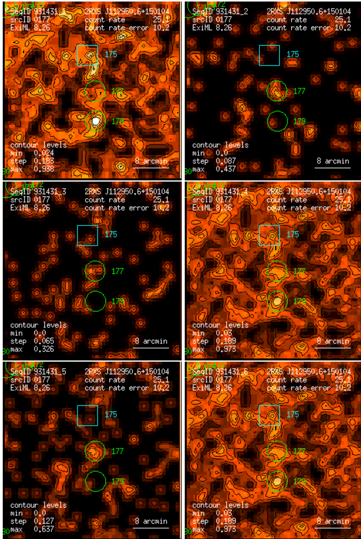
Figure 177: RASS 931431: detection 0177: band rate images, Gaussian filter: (1) PSPC channels 11 – 41, (2) 52 – 90, (3) 91 – 201, (4) 11 – 235, (5) 52 – 201, (6) 11 – 201. Broad band rates in counts/ks. Band rate contour levels in counts/ks/arcmin 2 .
