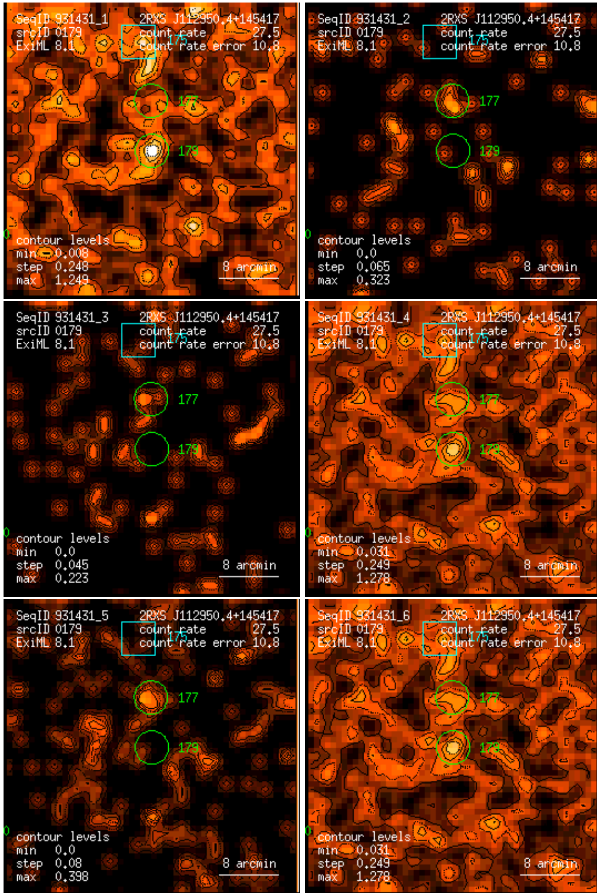
Figure 179: RASS 931431: detection 0179: band rate images, Gaussian filter: (1) PSPC channels 11 – 41, (2) 52 – 90, (3) 91 – 201, (4) 11 – 235, (5) 52 – 201, (6) 11 – 201. Broad band rates in counts/ks. Band rate contour levels in counts/ks/arcmin 2 .
