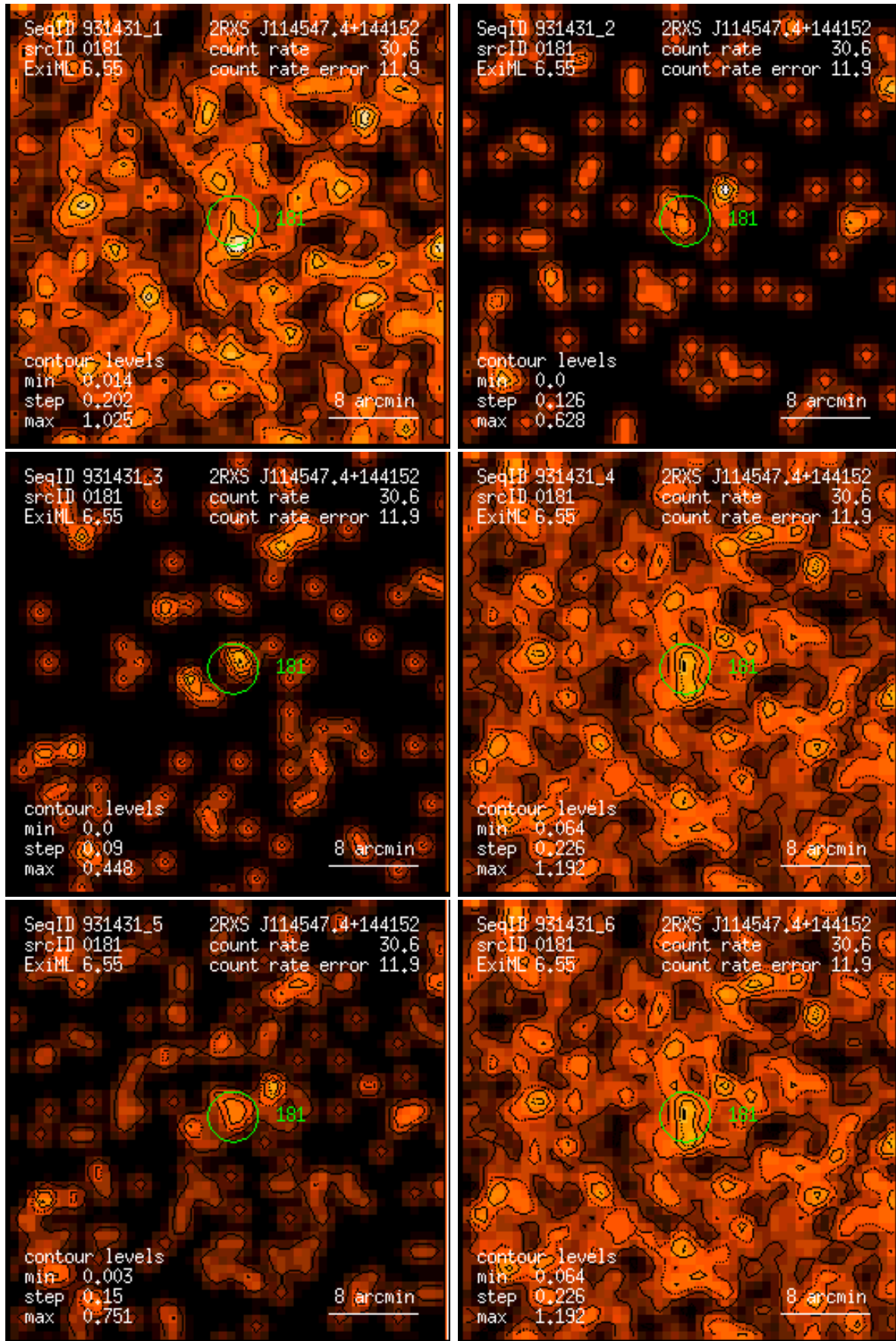
Figure 181: RASS 931431: detection 0181: band rate images, Gaussian filter: (1) PSPC channels 11 – 41, (2) 52 – 90, (3) 91 – 201, (4) 11 – 235, (5) 52 – 201, (6) 11 – 201. Broad band rates in counts/ks. Band rate contour levels in counts/ks/arcmin 2 .
