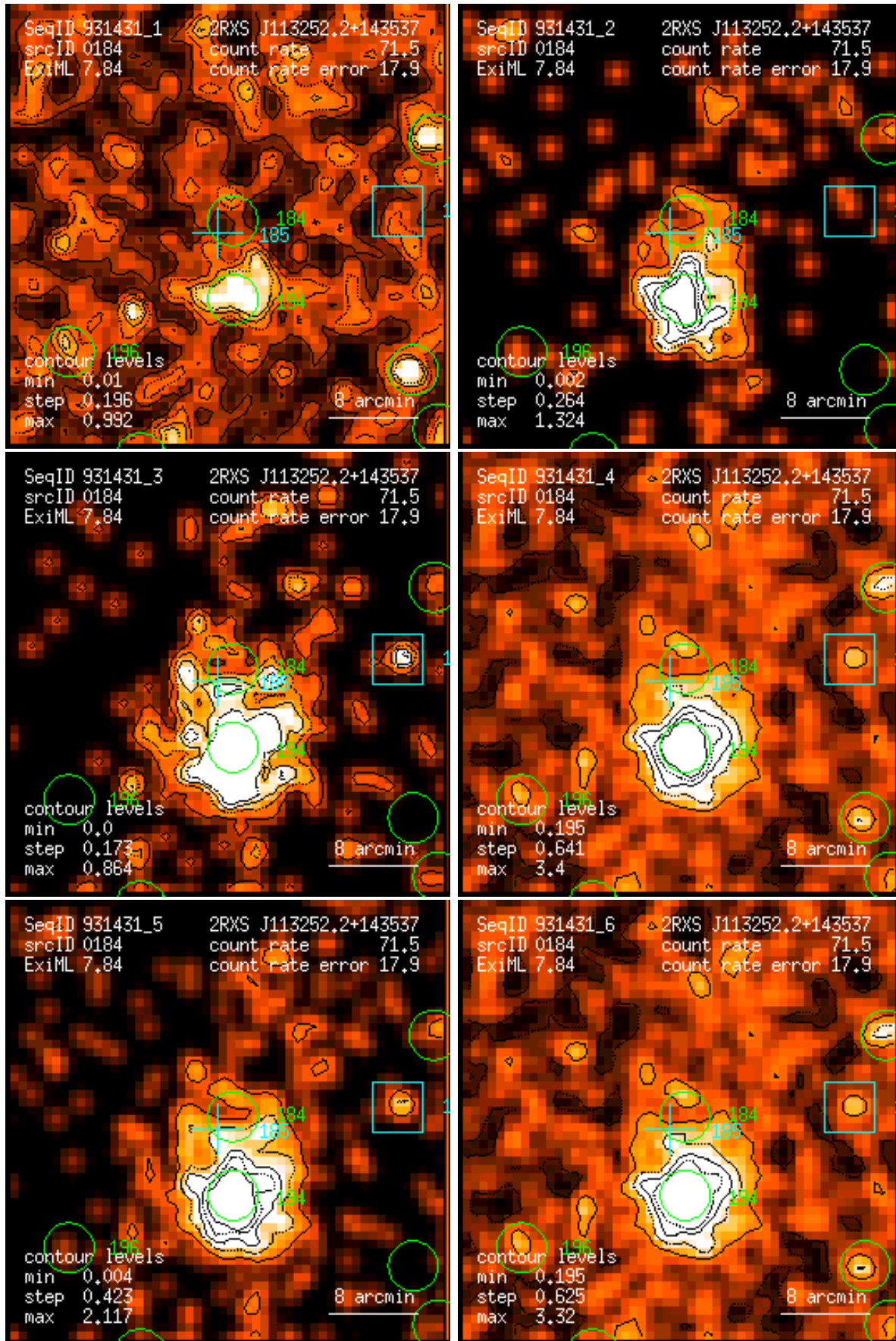
Figure 184: RASS 931431: detection 0184: band rate images, Gaussian filter: (1) PSPC channels 11 – 41, (2) 52 – 90, (3) 91 – 201, (4) 11 – 235, (5) 52 – 201, (6) 11 – 201. Broad band rates in counts/ks. Band rate contour levels in counts/ks/arcmin 2 .
