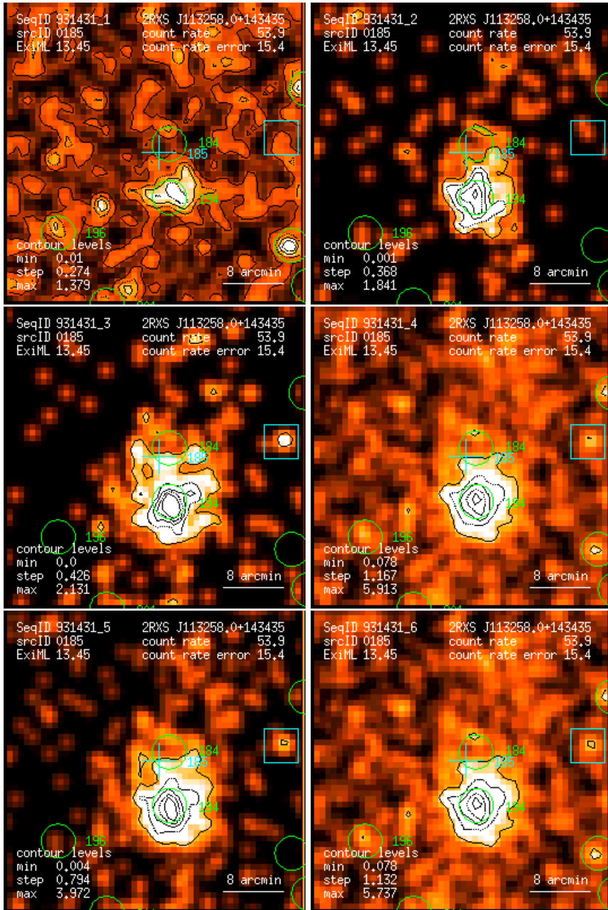
Figure 185: RASS 931431: detection 0185: band rate images, Gaussian filter: (1) PSPC channels 11 – 41, (2) 52 – 90, (3) 91 – 201, (4) 11 – 235, (5) 52 – 201, (6) 11 – 201. Broad band rates in counts/ks. Band rate contour levels in counts/ks/arcmin 2 .
