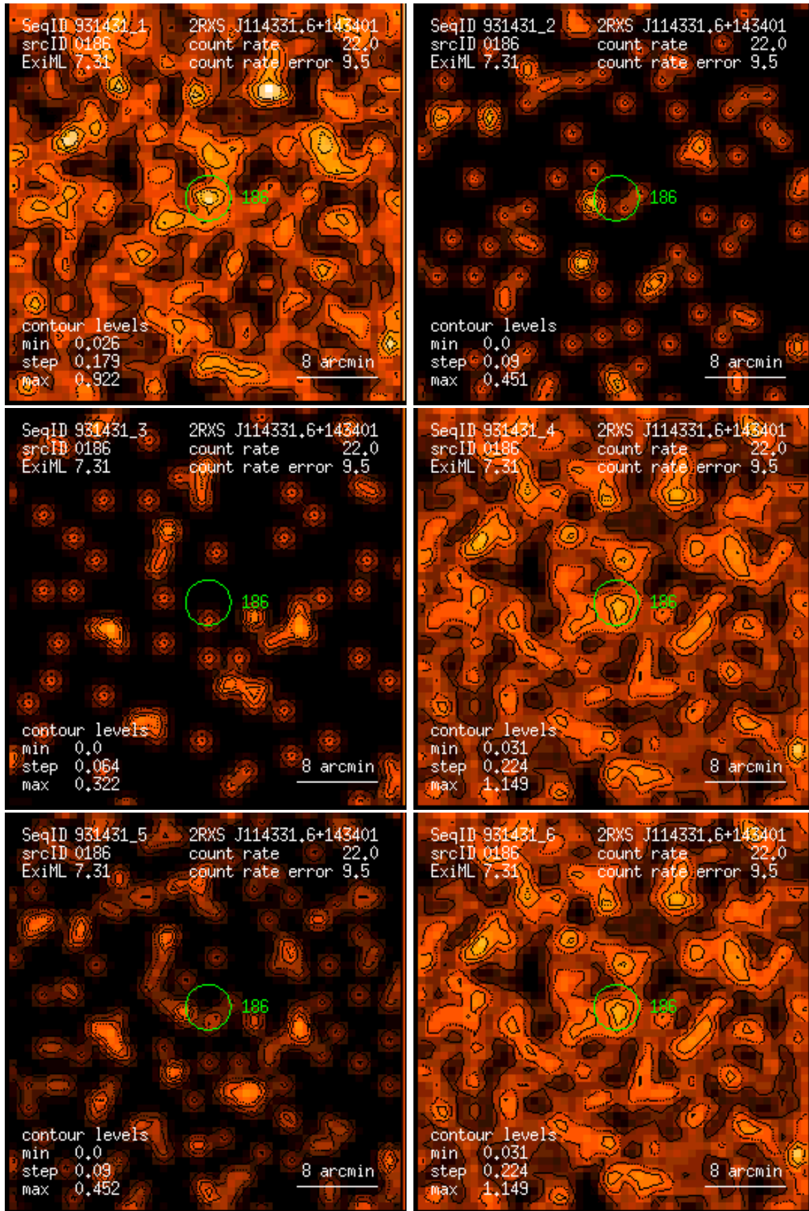
Figure 186: RASS 931431: detection 0186: band rate images, Gaussian filter: (1) PSPC channels 11 – 41, (2) 52 – 90, (3) 91 – 201, (4) 11 – 235, (5) 52 – 201, (6) 11 – 201. Broad band rates in counts/ks. Band rate contour levels in counts/ks/arcmin 2 .
