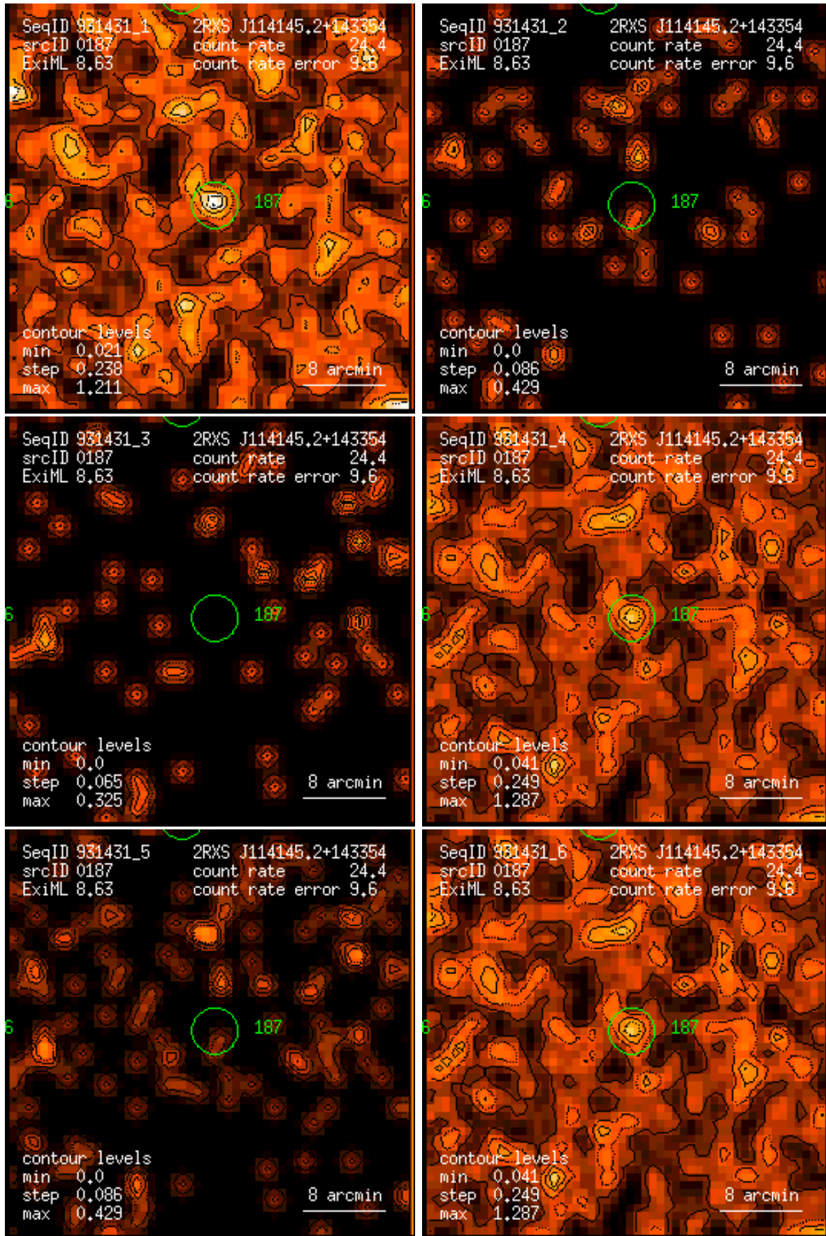
Figure 187: RASS 931431: detection 0187: band rate images, Gaussian filter: (1) PSPC channels 11 – 41, (2) 52 – 90, (3) 91 – 201, (4) 11 – 235, (5) 52 – 201, (6) 11 – 201. Broad band rates in counts/ks. Band rate contour levels in counts/ks/arcmin 2 .
