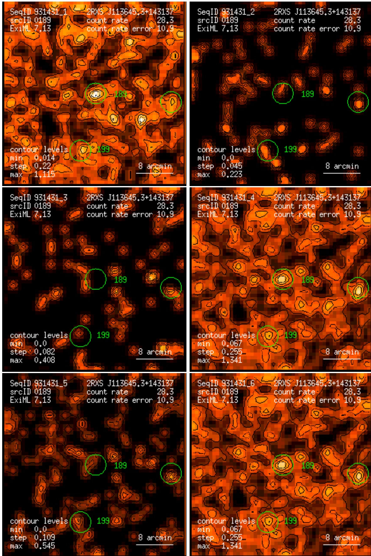
Figure 189: RASS 931431: detection 0189: band rate images, Gaussian filter: (1) PSPC channels 11 – 41, (2) 52 – 90, (3) 91 – 201, (4) 11 – 235, (5) 52 – 201, (6) 11 – 201. Broad band rates in counts/ks. Band rate contour levels in counts/ks/arcmin 2 .
