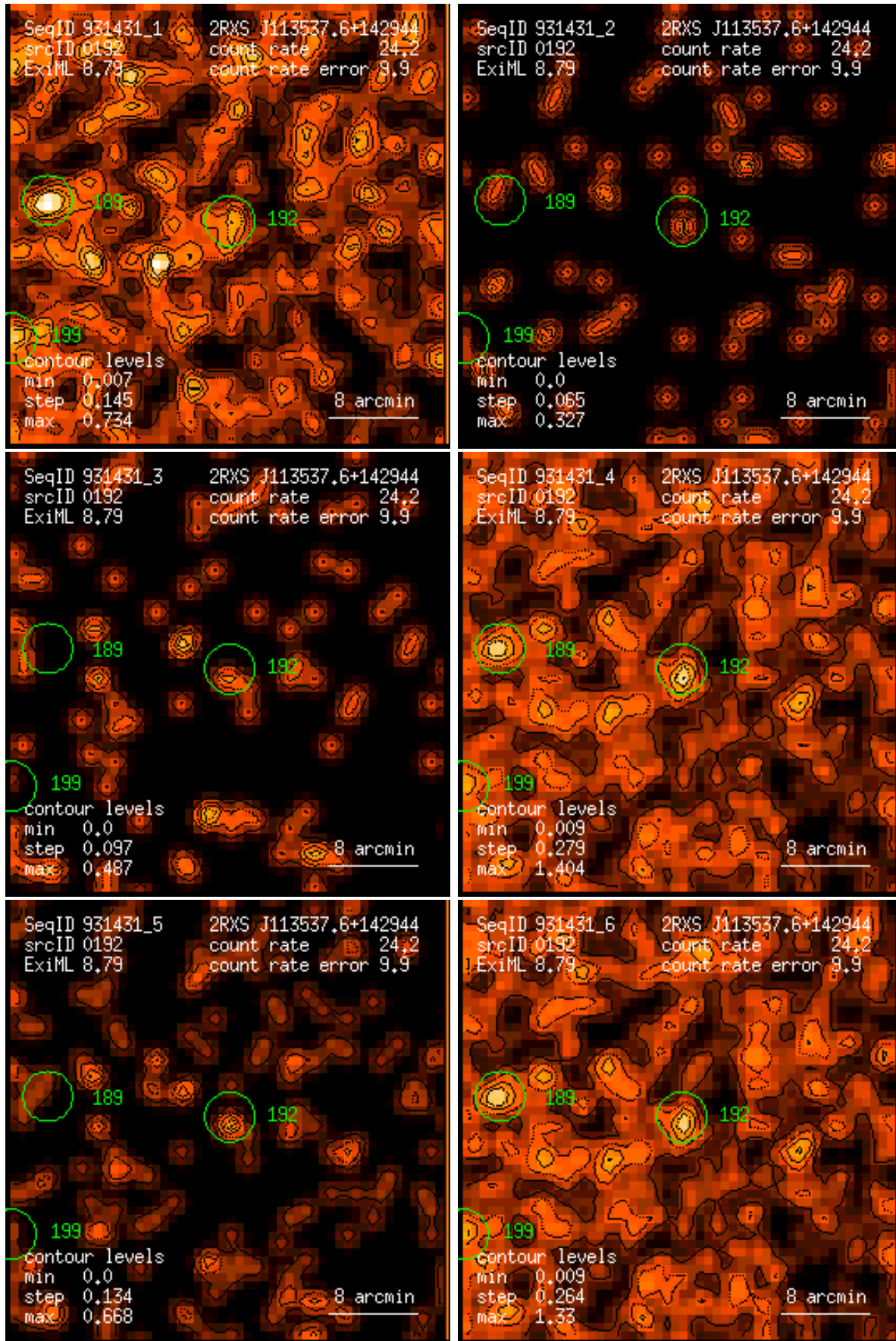
Figure 192: RASS 931431: detection 0192: band rate images, Gaussian filter: (1) PSPC channels 11 – 41, (2) 52 – 90, (3) 91 – 201, (4) 11 – 235, (5) 52 – 201, (6) 11 – 201. Broad band rates in counts/ks. Band rate contour levels in counts/ks/arcmin 2 .
