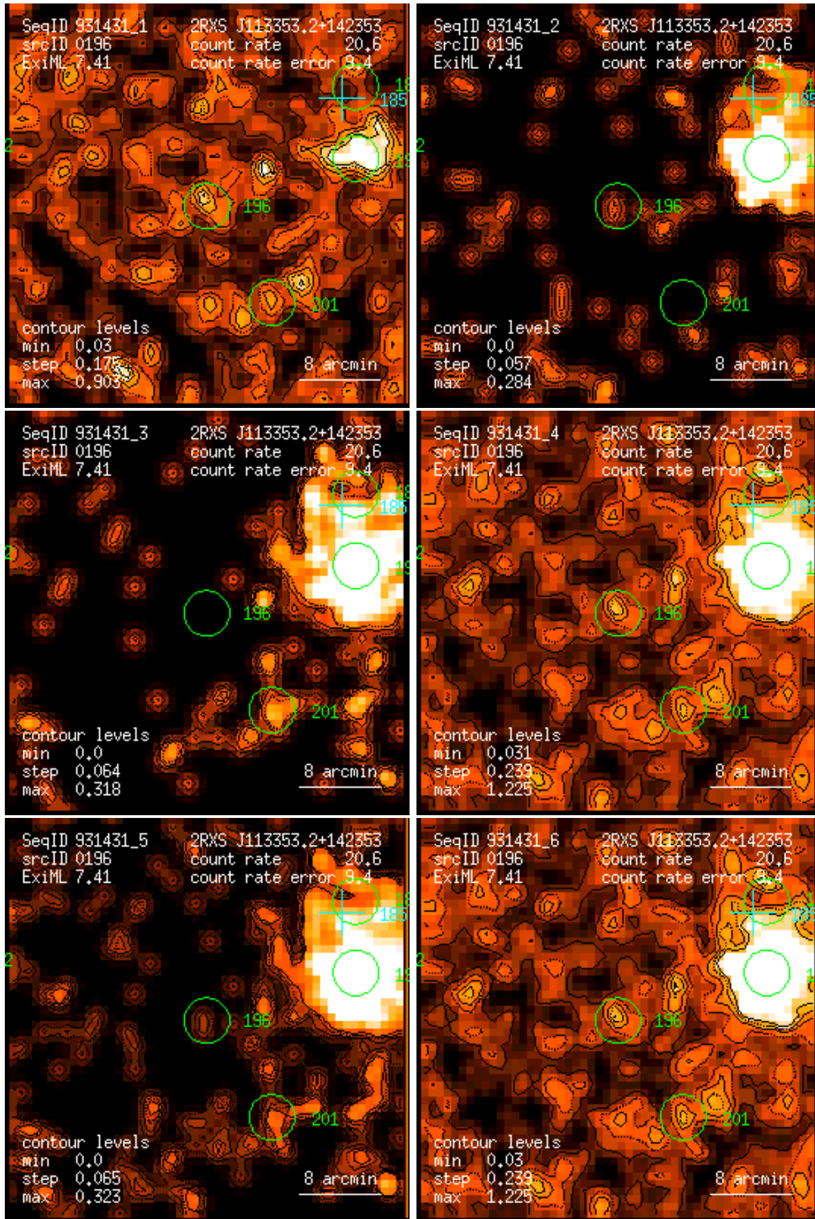
Figure 196: RASS 931431: detection 0196: band rate images, Gaussian filter: (1) PSPC channels 11 – 41, (2) 52 – 90, (3) 91 – 201, (4) 11 – 235, (5) 52 – 201, (6) 11 – 201. Broad band rates in counts/ks. Band rate contour levels in counts/ks/arcmin 2 .
