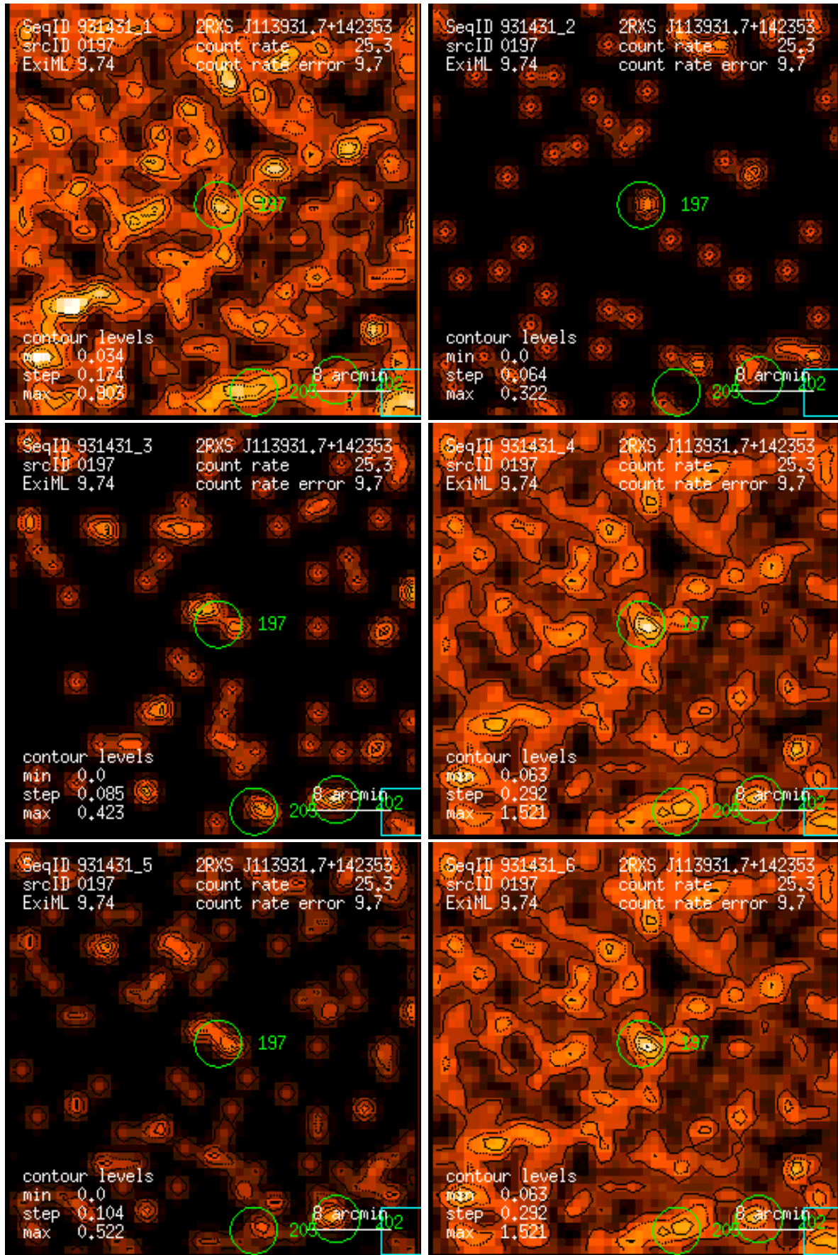
Figure 197: RASS 931431: detection 0197: band rate images, Gaussian filter: (1) PSPC channels 11 – 41, (2) 52 – 90, (3) 91 – 201, (4) 11 – 235, (5) 52 – 201, (6) 11 – 201. Broad band rates in counts/ks. Band rate contour levels in counts/ks/arcmin 2 .
